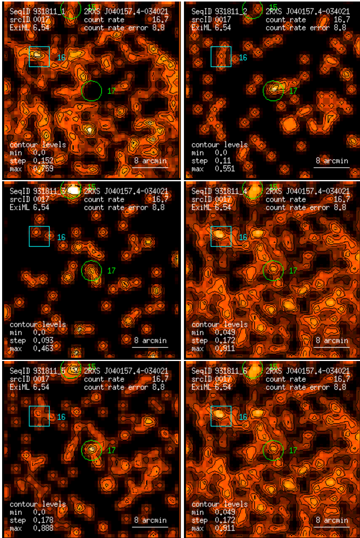
Figure 17: RASS 931811: detection 0017: band rate images, Gaussian filter: (1) PSPC channels 11 – 41, (2) 52 – 90, (3) 91 – 201, (4) 11 – 235, (5) 52 – 201, (6) 11 – 201. Broad band rates in counts/ks. Band rate contour levels in counts/ks/arcmin 2 .
