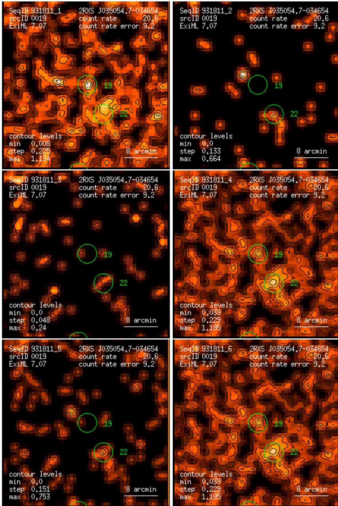
Figure 19: RASS 931811: detection 0019: band rate images, Gaussian filter: (1) PSPC channels 11 – 41, (2) 52 – 90, (3) 91 – 201, (4) 11 – 235, (5) 52 – 201, (6) 11 – 201. Broad band rates in counts/ks. Band rate contour levels in counts/ks/arcmin 2 .
