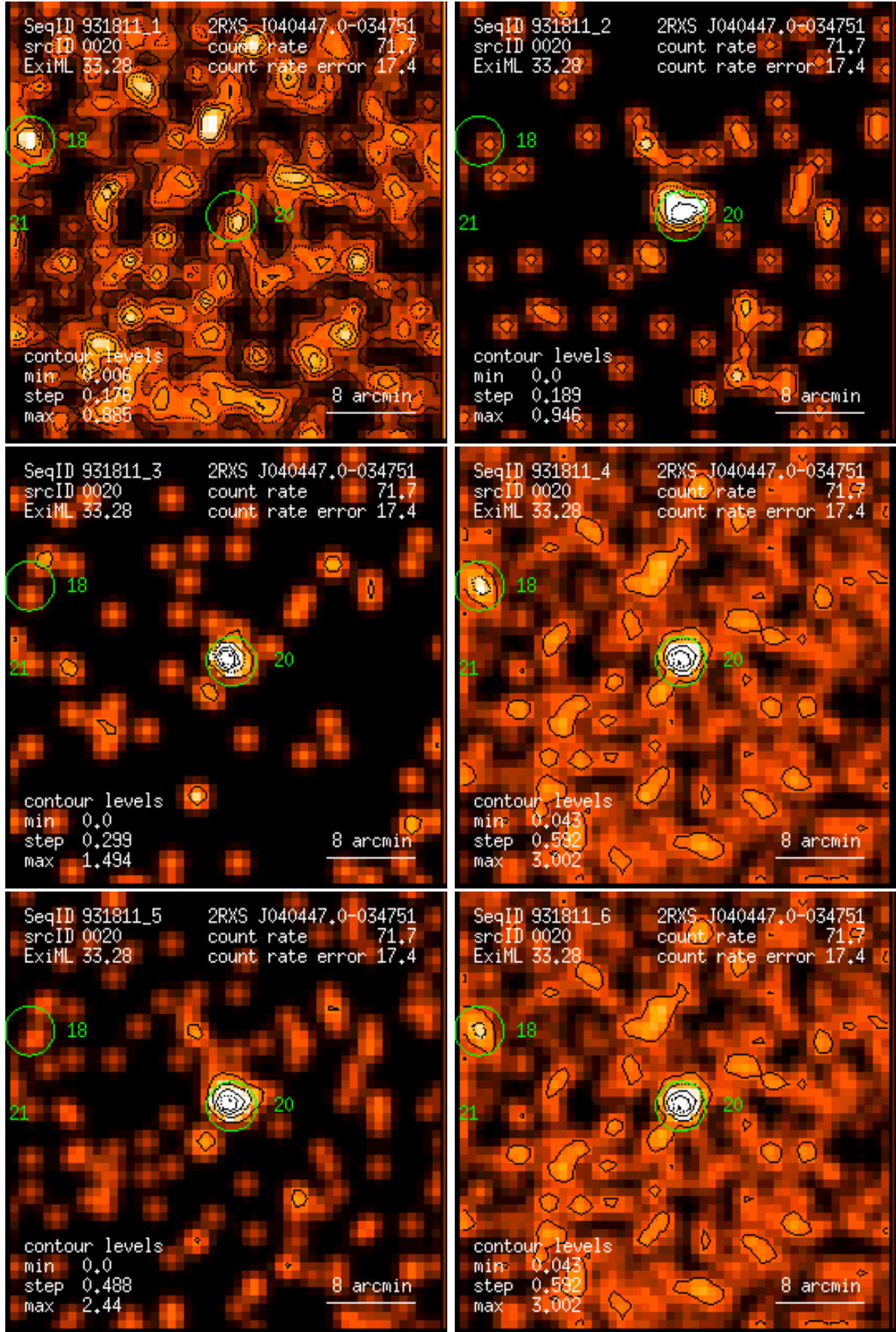
Figure 20: RASS 931811: detection 0020: band rate images, Gaussian filter: (1) PSPC channels 11 – 41, (2) 52 – 90, (3) 91 – 201, (4) 11 – 235, (5) 52 – 201, (6) 11 – 201. Broad band rates in counts/ks. Band rate contour levels in counts/ks/arcmin 2 .
