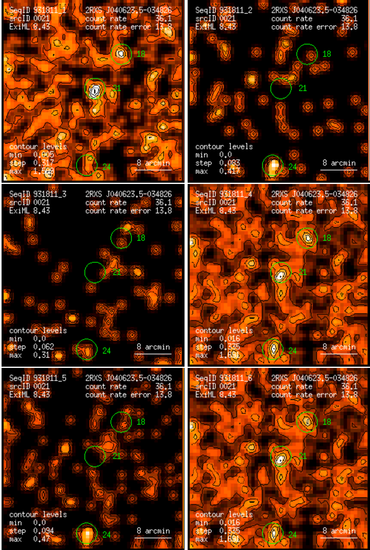
Figure 21: RASS 931811: detection 0021: band rate images, Gaussian filter: (1) PSPC channels 11 – 41, (2) 52 – 90, (3) 91 – 201, (4) 11 – 235, (5) 52 – 201, (6) 11 – 201. Broad band rates in counts/ks. Band rate contour levels in counts/ks/arcmin 2 .
