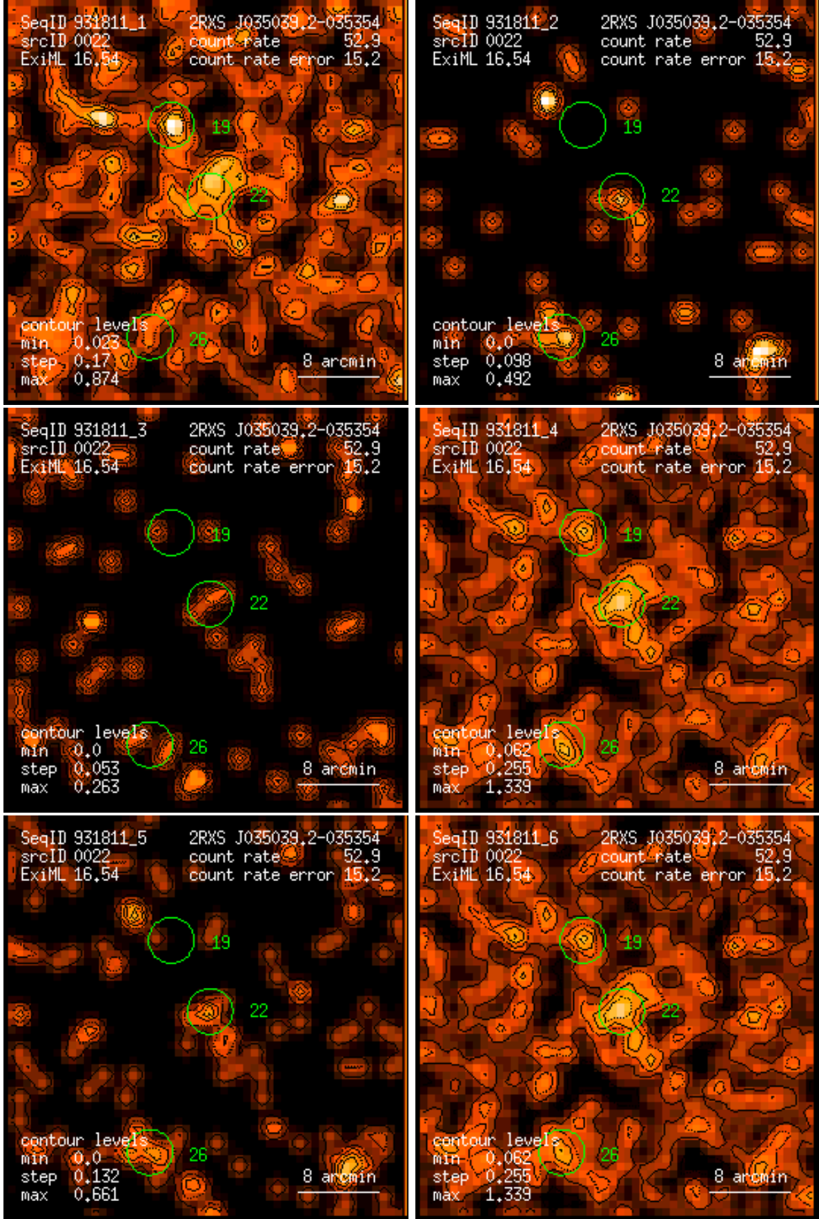
Figure 22: RASS 931811: detection 0022: band rate images, Gaussian filter: (1) PSPC channels 11 – 41, (2) 52 – 90, (3) 91 – 201, (4) 11 – 235, (5) 52 – 201, (6) 11 – 201. Broad band rates in counts/ks. Band rate contour levels in counts/ks/arcmin 2 .
