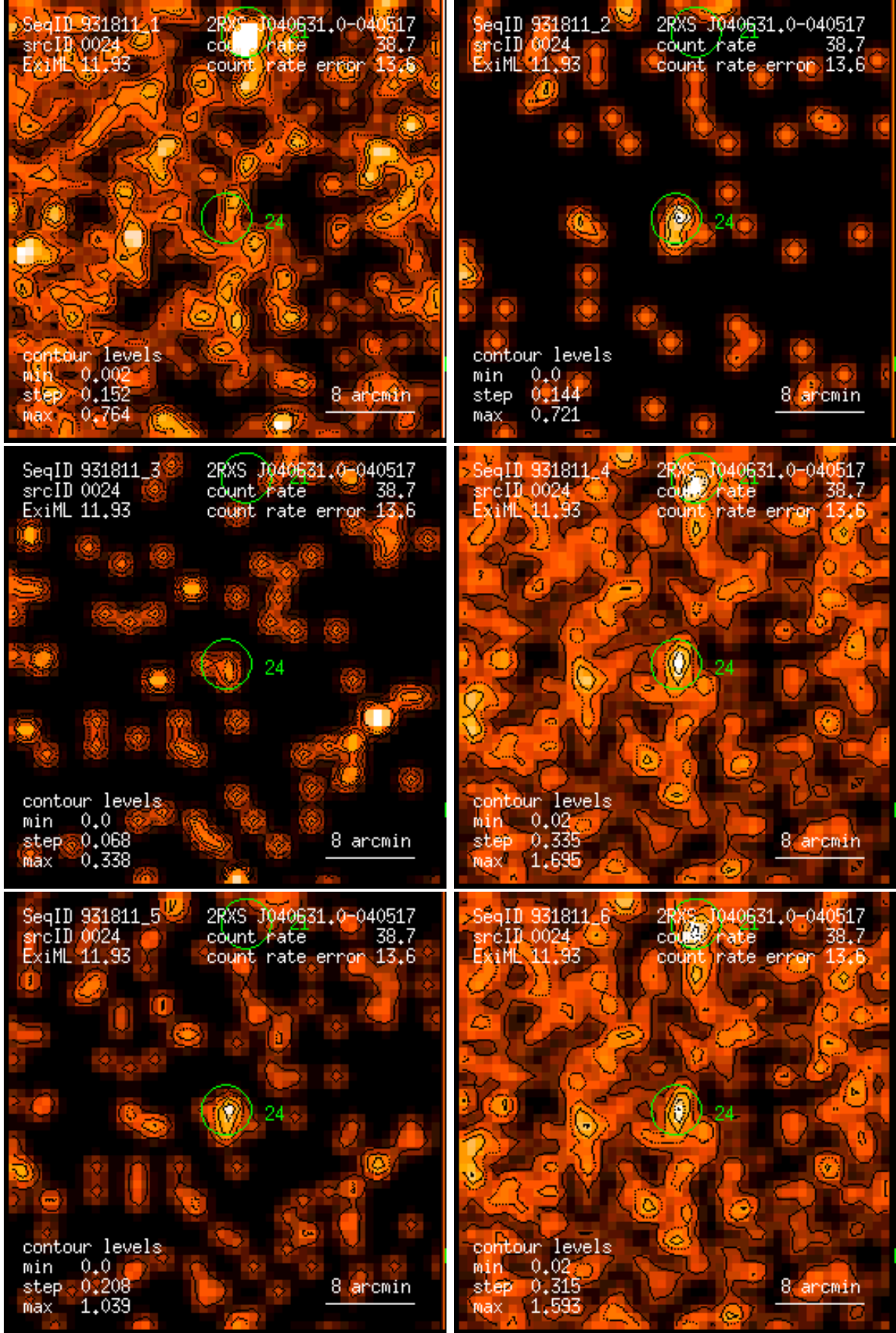
Figure 24: RASS 931811: detection 0024: band rate images, Gaussian filter: (1) PSPC channels 11 – 41, (2) 52 – 90, (3) 91 – 201, (4) 11 – 235, (5) 52 – 201, (6) 11 – 201. Broad band rates in counts/ks. Band rate contour levels in counts/ks/arcmin 2 .
