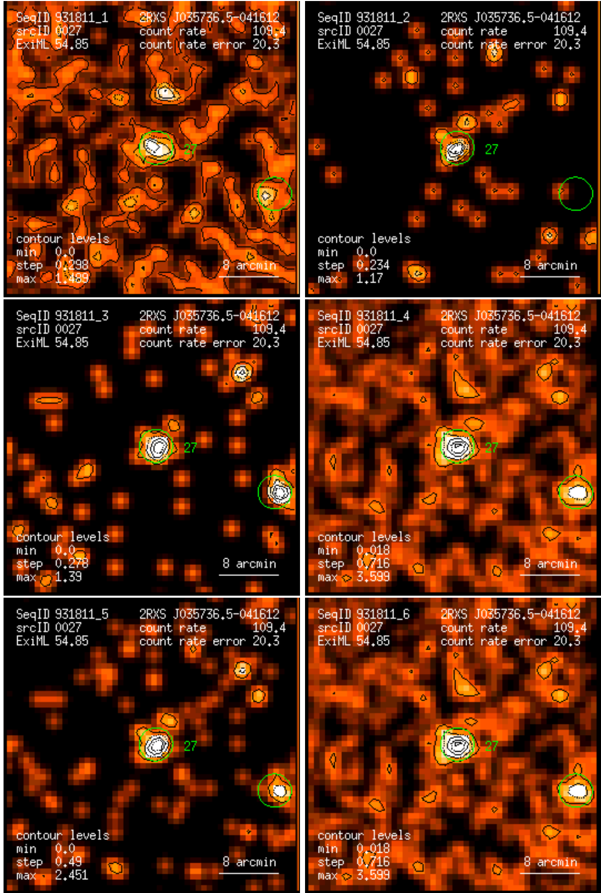
Figure 27: RASS 931811: detection 0027: band rate images, Gaussian filter: (1) PSPC channels 11 – 41, (2) 52 – 90, (3) 91 – 201, (4) 11 – 235, (5) 52 – 201, (6) 11 – 201. Broad band rates in counts/ks. Band rate contour levels in counts/ks/arcmin 2 .
