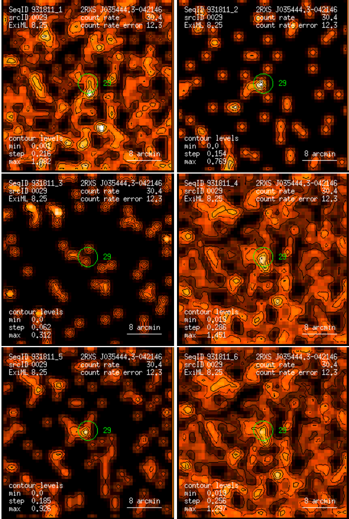
Figure 29: RASS 931811: detection 0029: band rate images, Gaussian filter: (1) PSPC channels 11 – 41, (2) 52 – 90, (3) 91 – 201, (4) 11 – 235, (5) 52 – 201, (6) 11 – 201. Broad band rates in counts/ks. Band rate contour levels in counts/ks/arcmin 2 .
