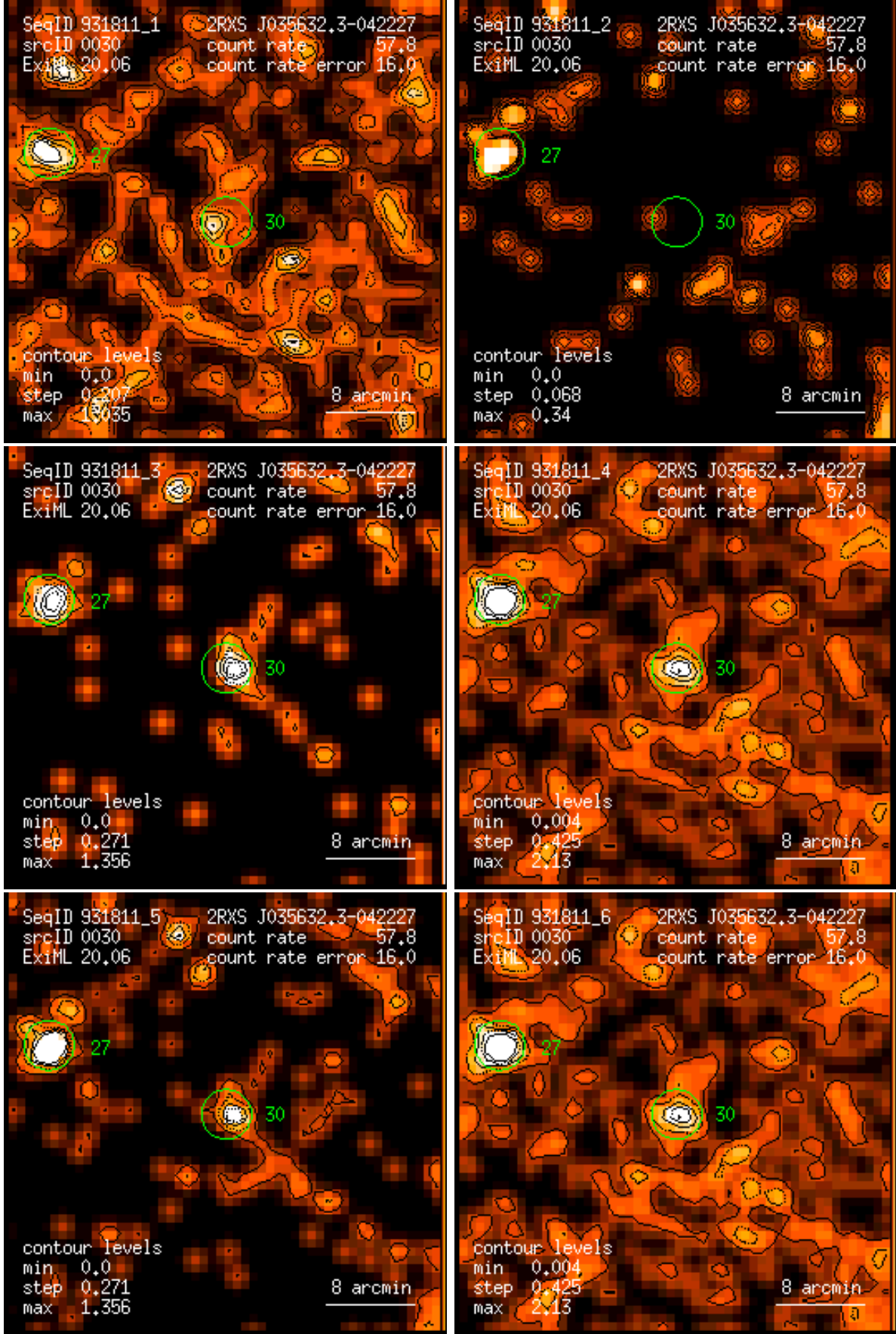
Figure 30: RASS 931811: detection 0030: band rate images, Gaussian filter: (1) PSPC channels 11 – 41, (2) 52 – 90, (3) 91 – 201, (4) 11 – 235, (5) 52 – 201, (6) 11 – 201. Broad band rates in counts/ks. Band rate contour levels in counts/ks/arcmin 2 .
