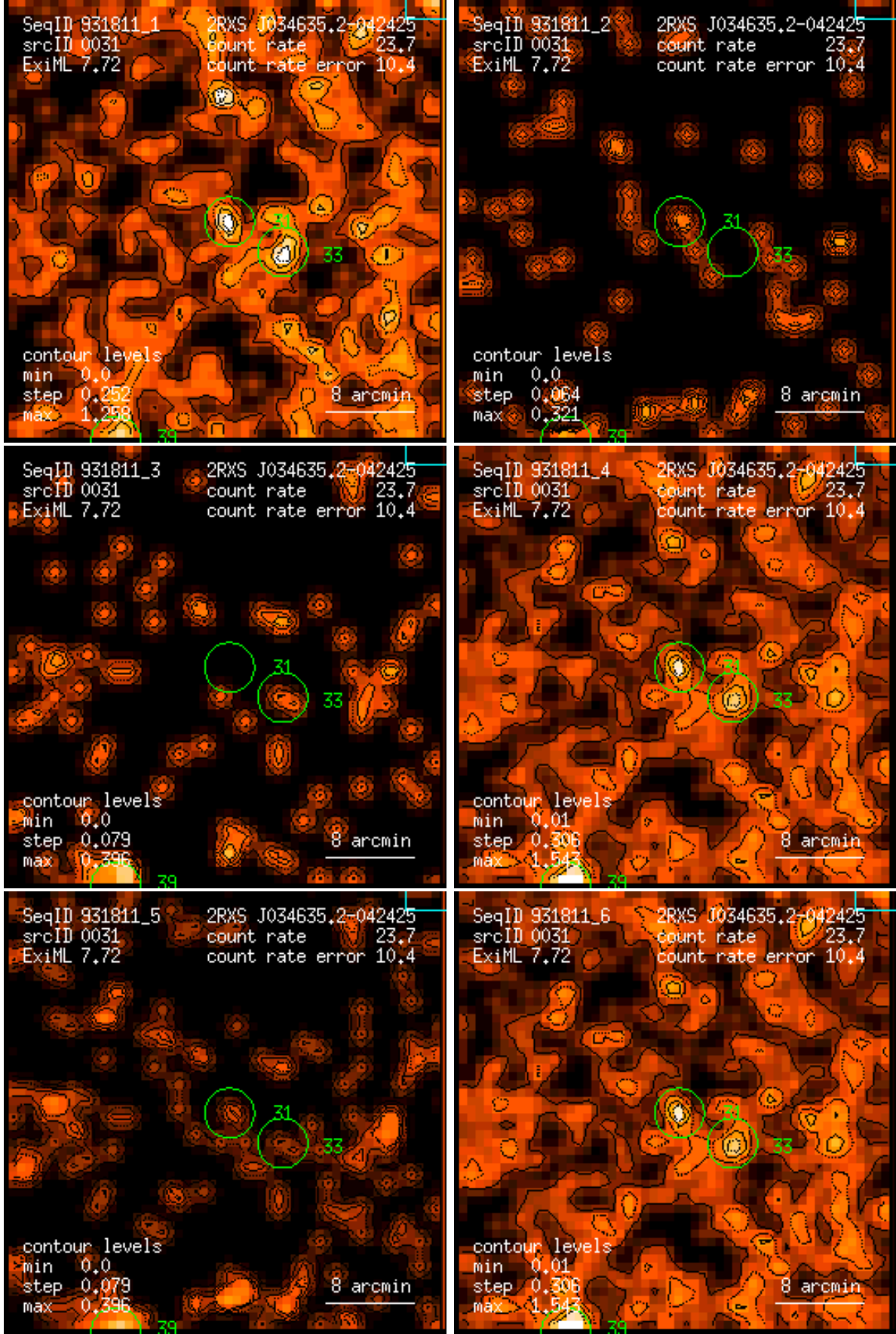
Figure 31: RASS 931811: detection 0031: band rate images, Gaussian filter: (1) PSPC channels 11 – 41, (2) 52 – 90, (3) 91 – 201, (4) 11 – 235, (5) 52 – 201, (6) 11 – 201. Broad band rates in counts/ks. Band rate contour levels in counts/ks/arcmin 2 .
