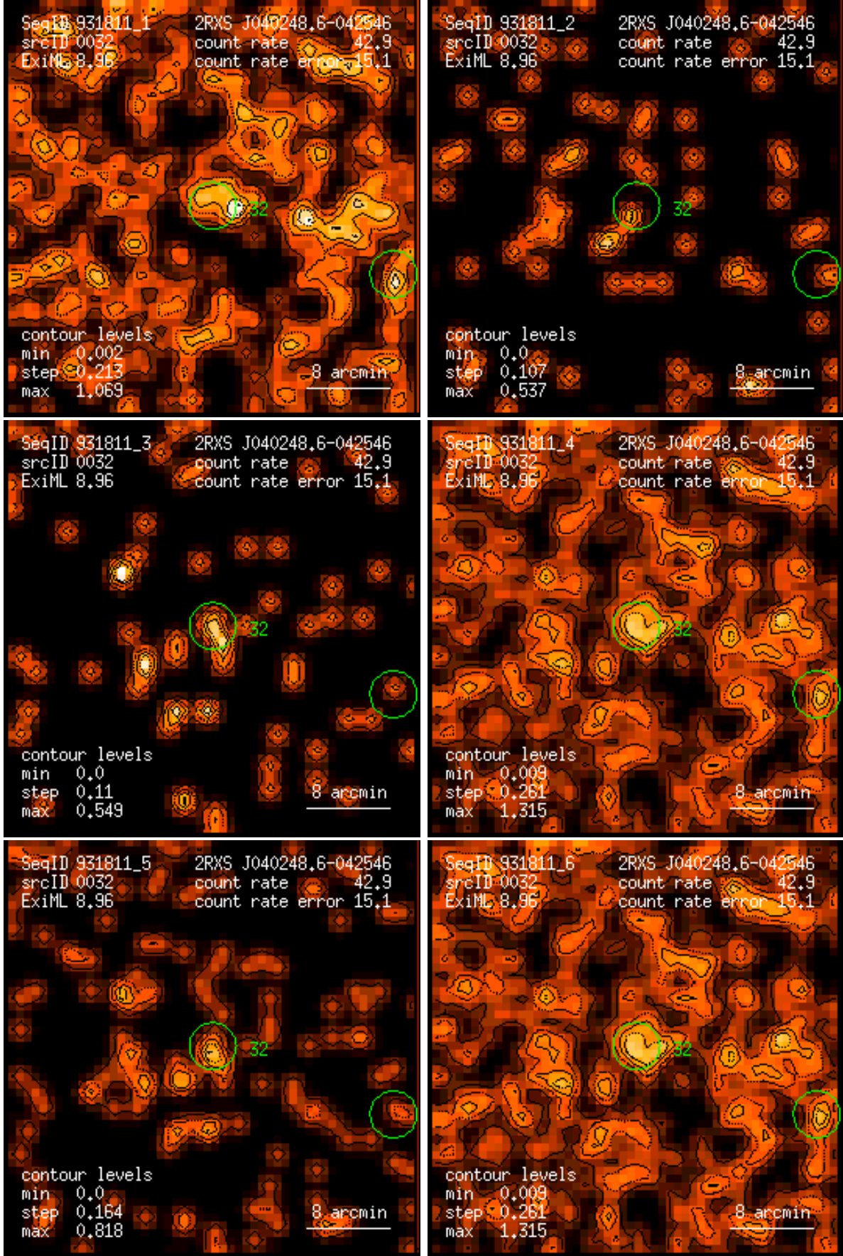
Figure 32: RASS 931811: detection 0032: band rate images, Gaussian filter: (1) PSPC channels 11 – 41, (2) 52 – 90, (3) 91 – 201, (4) 11 – 235, (5) 52 – 201, (6) 11 – 201. Broad band rates in counts/ks. Band rate contour levels in counts/ks/arcmin 2 .
