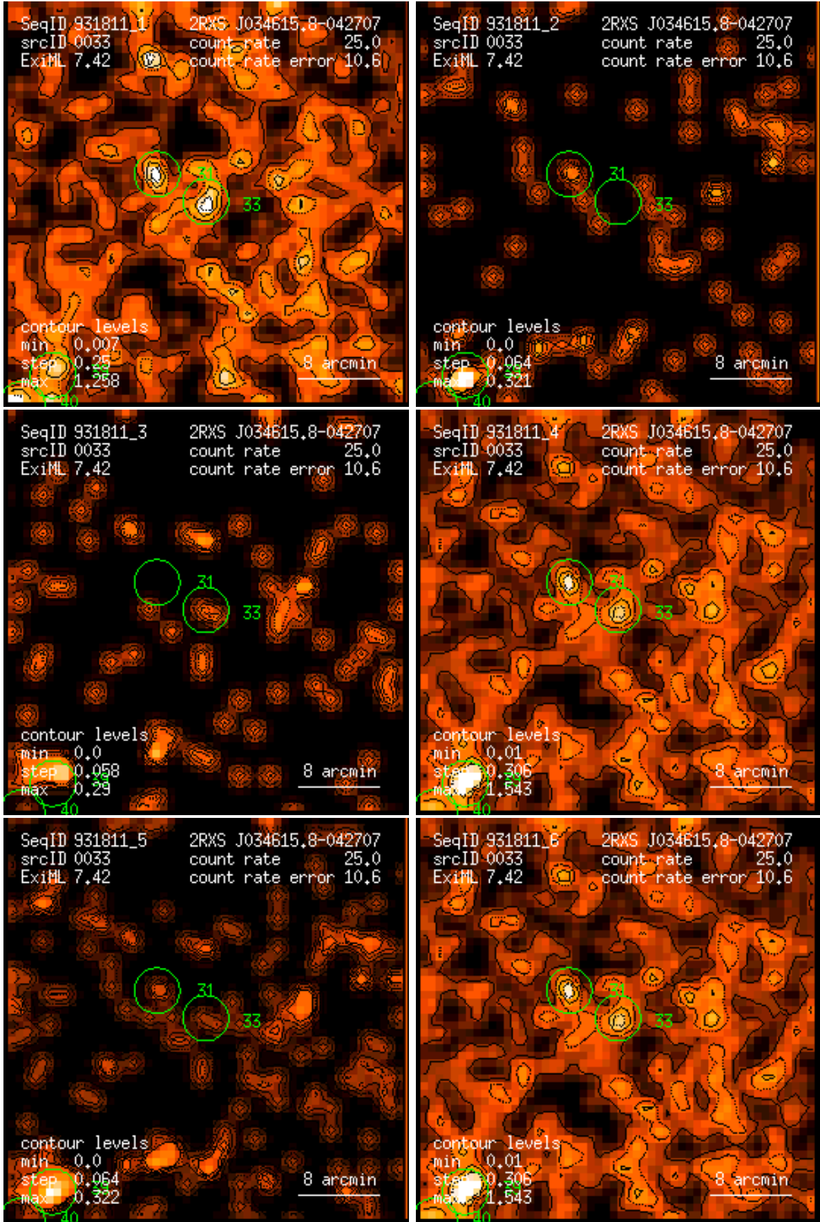
Figure 33: RASS 931811: detection 0033: band rate images, Gaussian filter: (1) PSPC channels 11 – 41, (2) 52 – 90, (3) 91 – 201, (4) 11 – 235, (5) 52 – 201, (6) 11 – 201. Broad band rates in counts/ks. Band rate contour levels in counts/ks/arcmin 2 .
