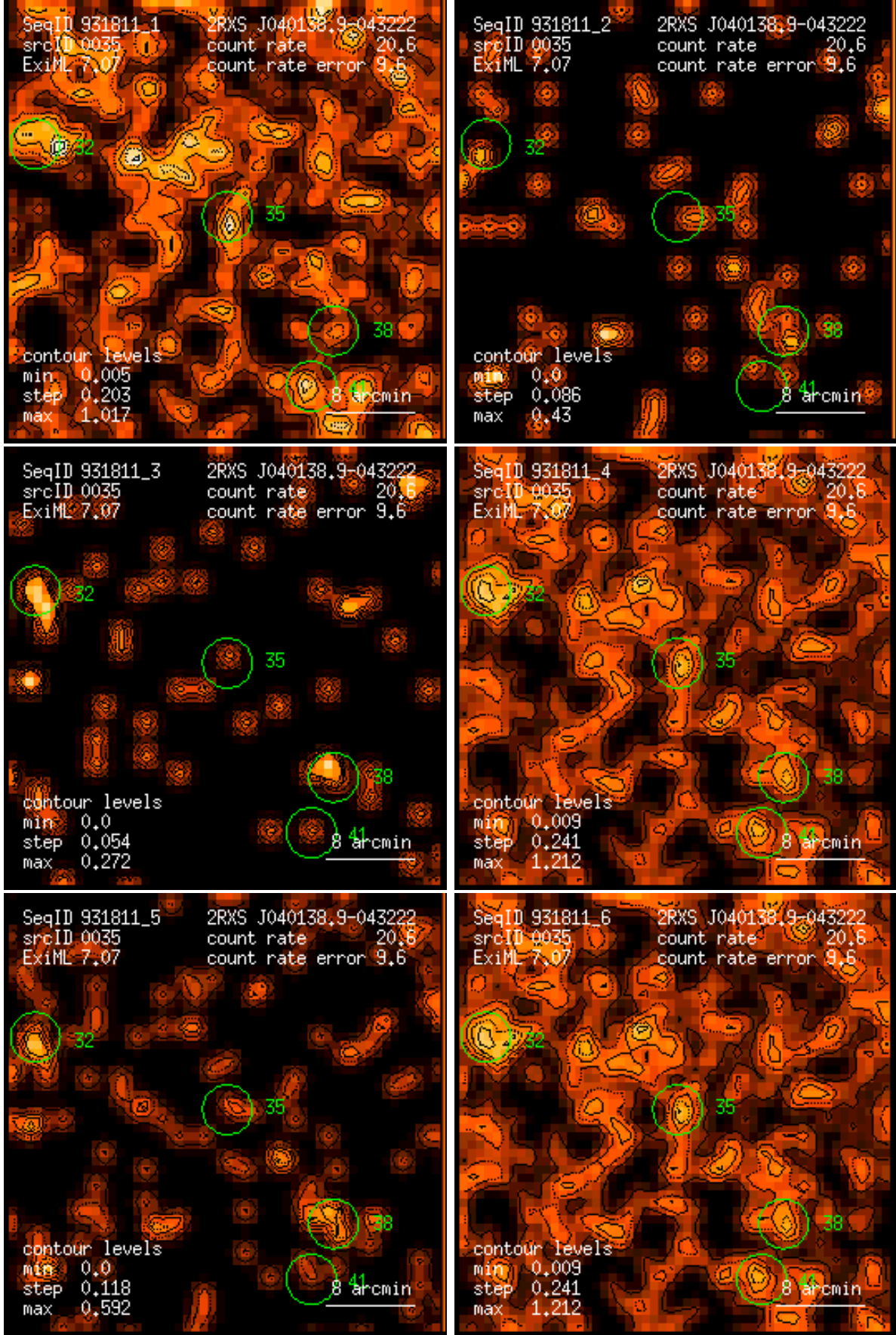
Figure 35: RASS 931811: detection 0035: band rate images, Gaussian filter: (1) PSPC channels 11 – 41, (2) 52 – 90, (3) 91 – 201, (4) 11 – 235, (5) 52 – 201, (6) 11 – 201. Broad band rates in counts/ks. Band rate contour levels in counts/ks/arcmin 2 .
