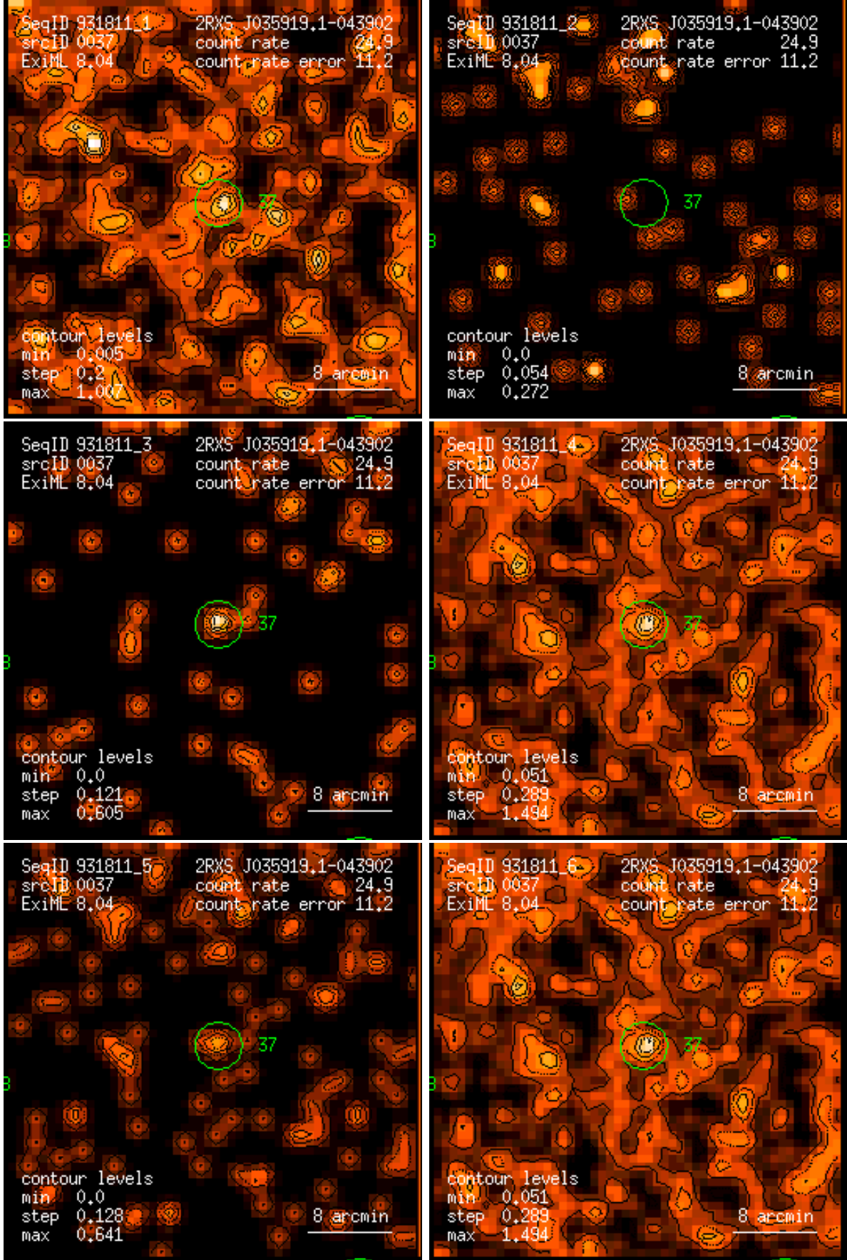
Figure 37: RASS 931811: detection 0037: band rate images, Gaussian filter: (1) PSPC channels 11 – 41, (2) 52 – 90, (3) 91 – 201, (4) 11 – 235, (5) 52 – 201, (6) 11 – 201. Broad band rates in counts/ks. Band rate contour levels in counts/ks/arcmin 2 .
