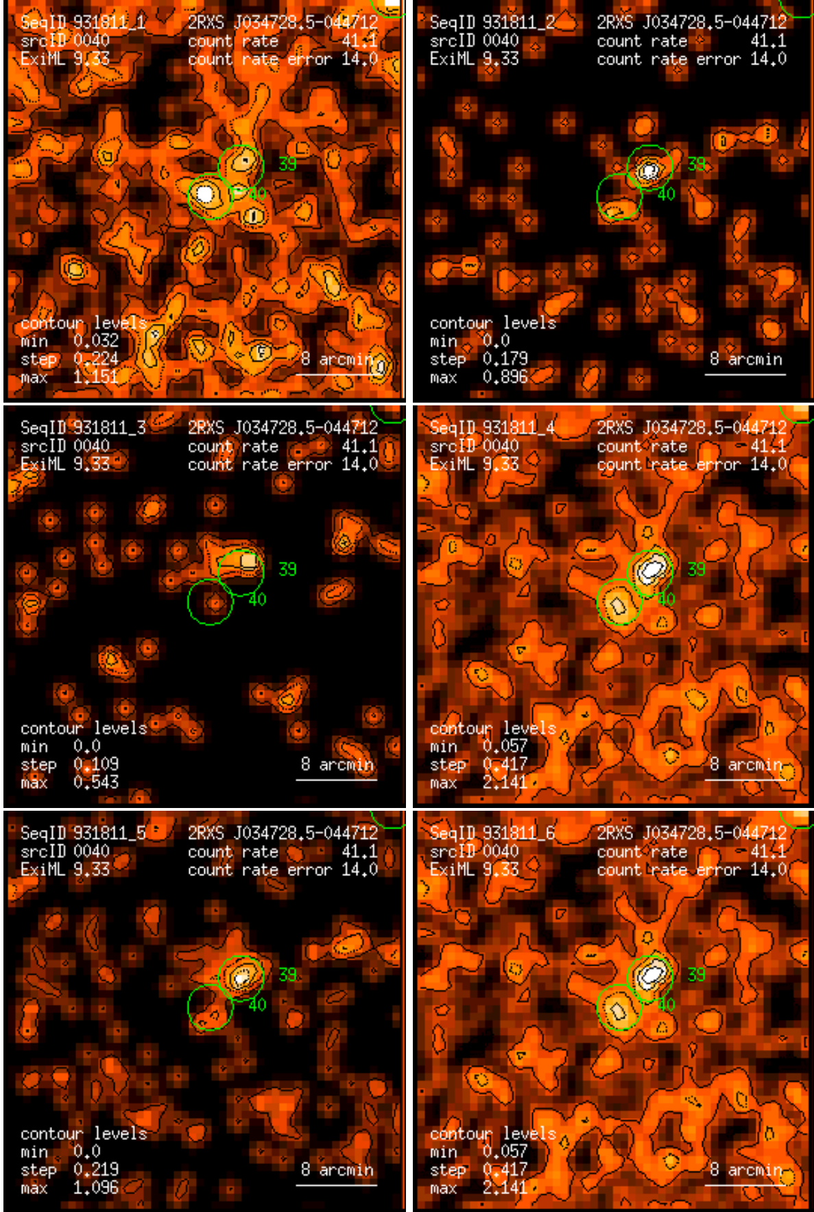
Figure 40: RASS 931811: detection 0040: band rate images, Gaussian filter: (1) PSPC channels 11 – 41, (2) 52 – 90, (3) 91 – 201, (4) 11 – 235, (5) 52 – 201, (6) 11 – 201. Broad band rates in counts/ks. Band rate contour levels in counts/ks/arcmin 2 .
