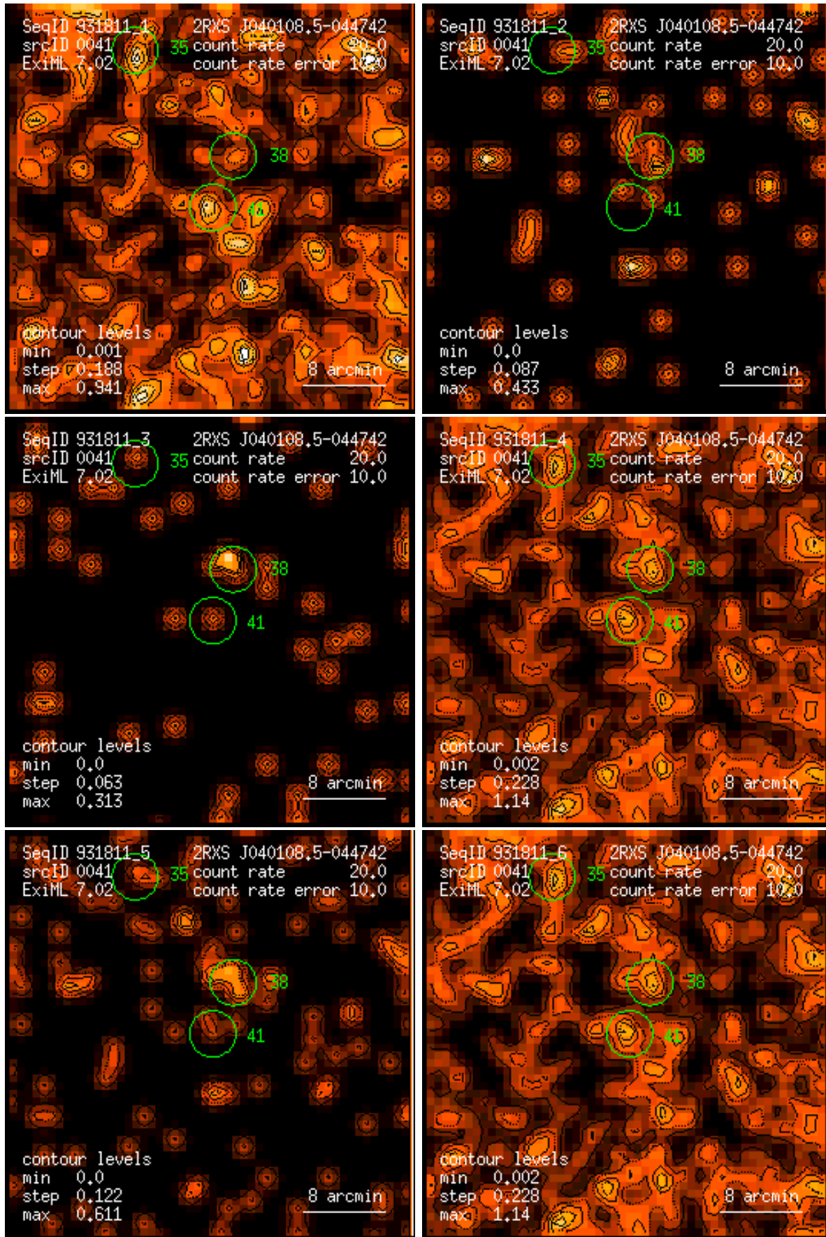
Figure 41: RASS 931811: detection 0041: band rate images, Gaussian filter: (1) PSPC channels 11 – 41, (2) 52 – 90, (3) 91 – 201, (4) 11 – 235, (5) 52 – 201, (6) 11 – 201. Broad band rates in counts/ks. Band rate contour levels in counts/ks/arcmin 2 .
