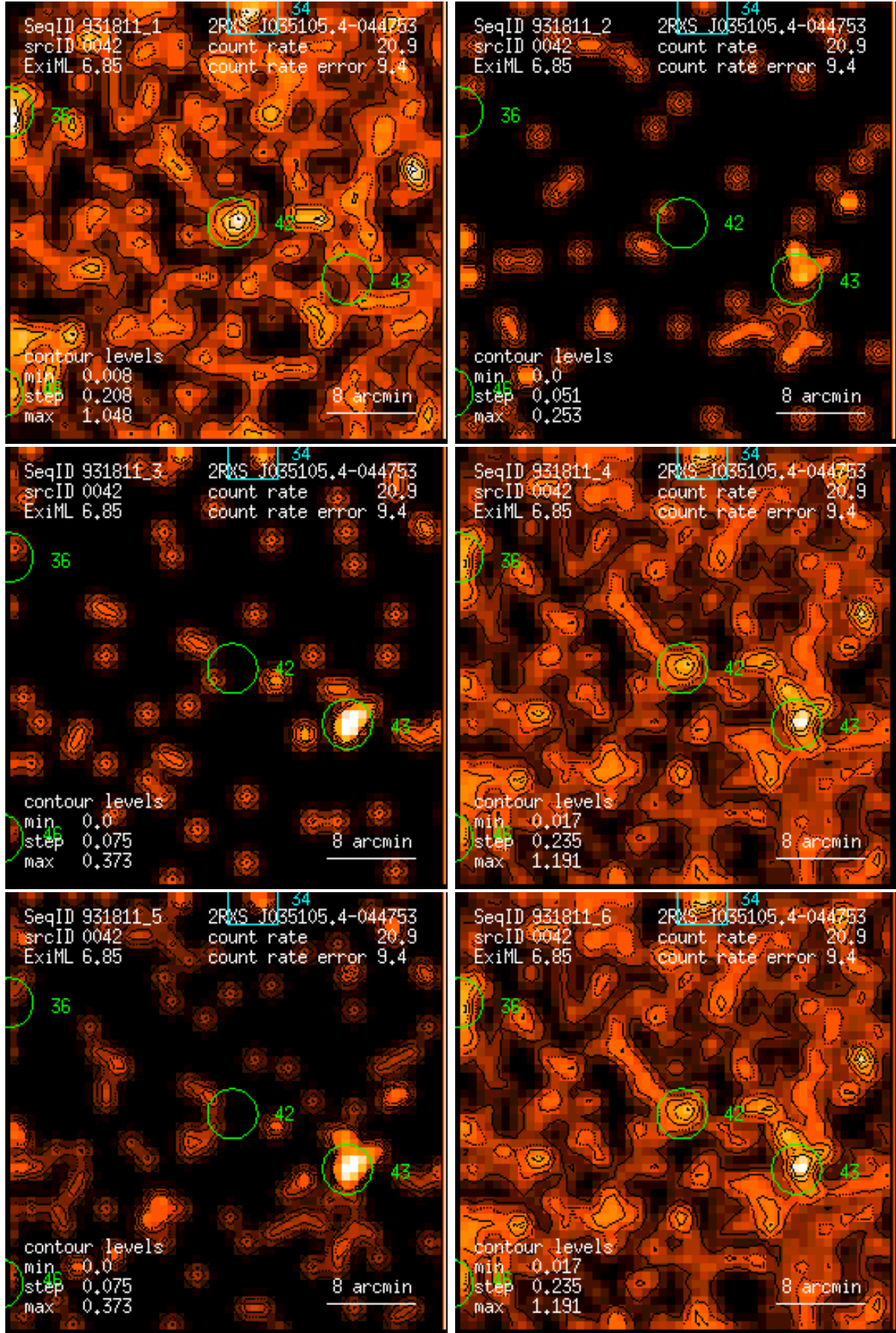
Figure 42: RASS 931811: detection 0042: band rate images, Gaussian filter: (1) PSPC channels 11 – 41, (2) 52 – 90, (3) 91 – 201, (4) 11 – 235, (5) 52 – 201, (6) 11 – 201. Broad band rates in counts/ks. Band rate contour levels in counts/ks/arcmin 2 .
