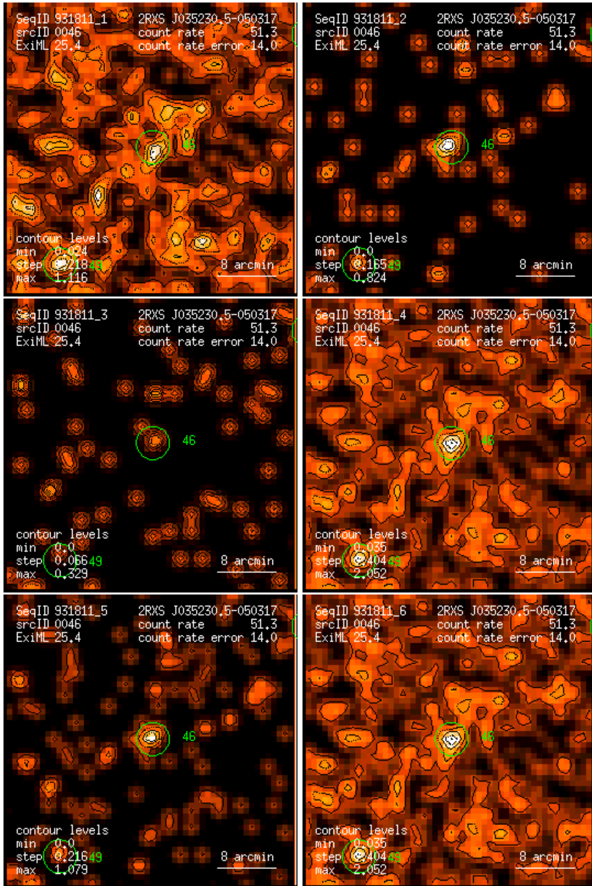
Figure 46: RASS 931811: detection 0046: band rate images, Gaussian filter: (1) PSPC channels 11 – 41, (2) 52 – 90, (3) 91 – 201, (4) 11 – 235, (5) 52 – 201, (6) 11 – 201. Broad band rates in counts/ks. Band rate contour levels in counts/ks/arcmin 2 .
