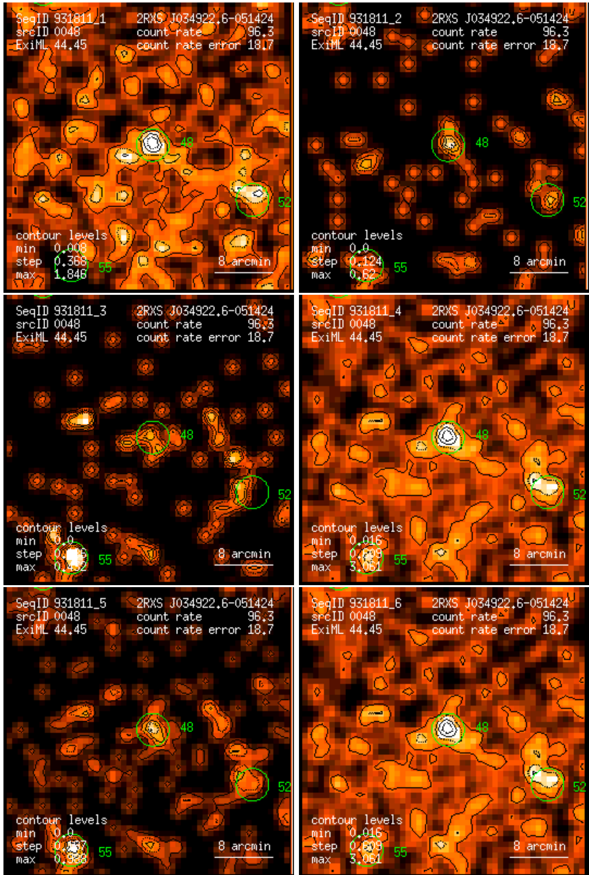
Figure 48: RASS 931811: detection 0048: band rate images, Gaussian filter: (1) PSPC channels 11 – 41, (2) 52 – 90, (3) 91 – 201, (4) 11 – 235, (5) 52 – 201, (6) 11 – 201. Broad band rates in counts/ks. Band rate contour levels in counts/ks/arcmin 2 .
