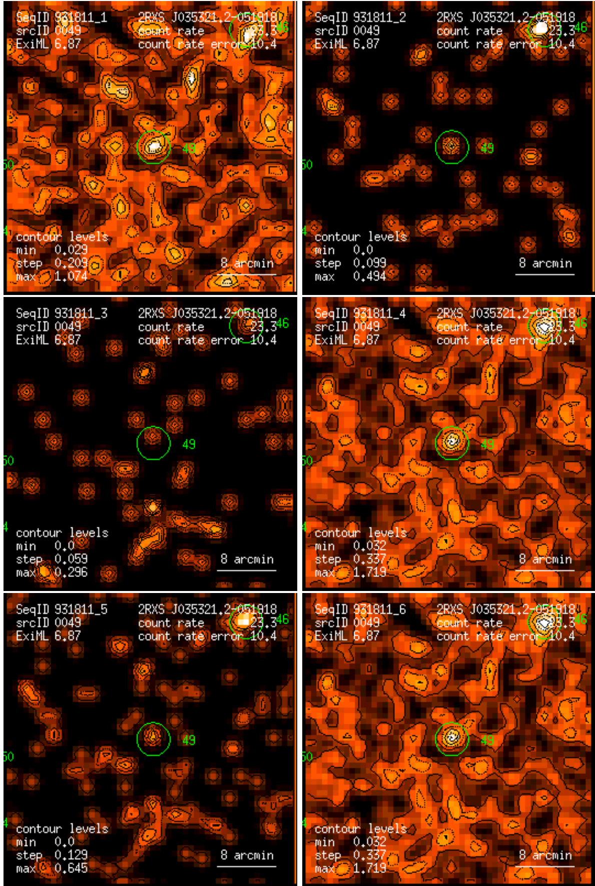
Figure 49: RASS 931811: detection 0049: band rate images, Gaussian filter: (1) PSPC channels 11 – 41, (2) 52 – 90, (3) 91 – 201, (4) 11 – 235, (5) 52 – 201, (6) 11 – 201. Broad band rates in counts/ks. Band rate contour levels in counts/ks/arcmin 2 .
