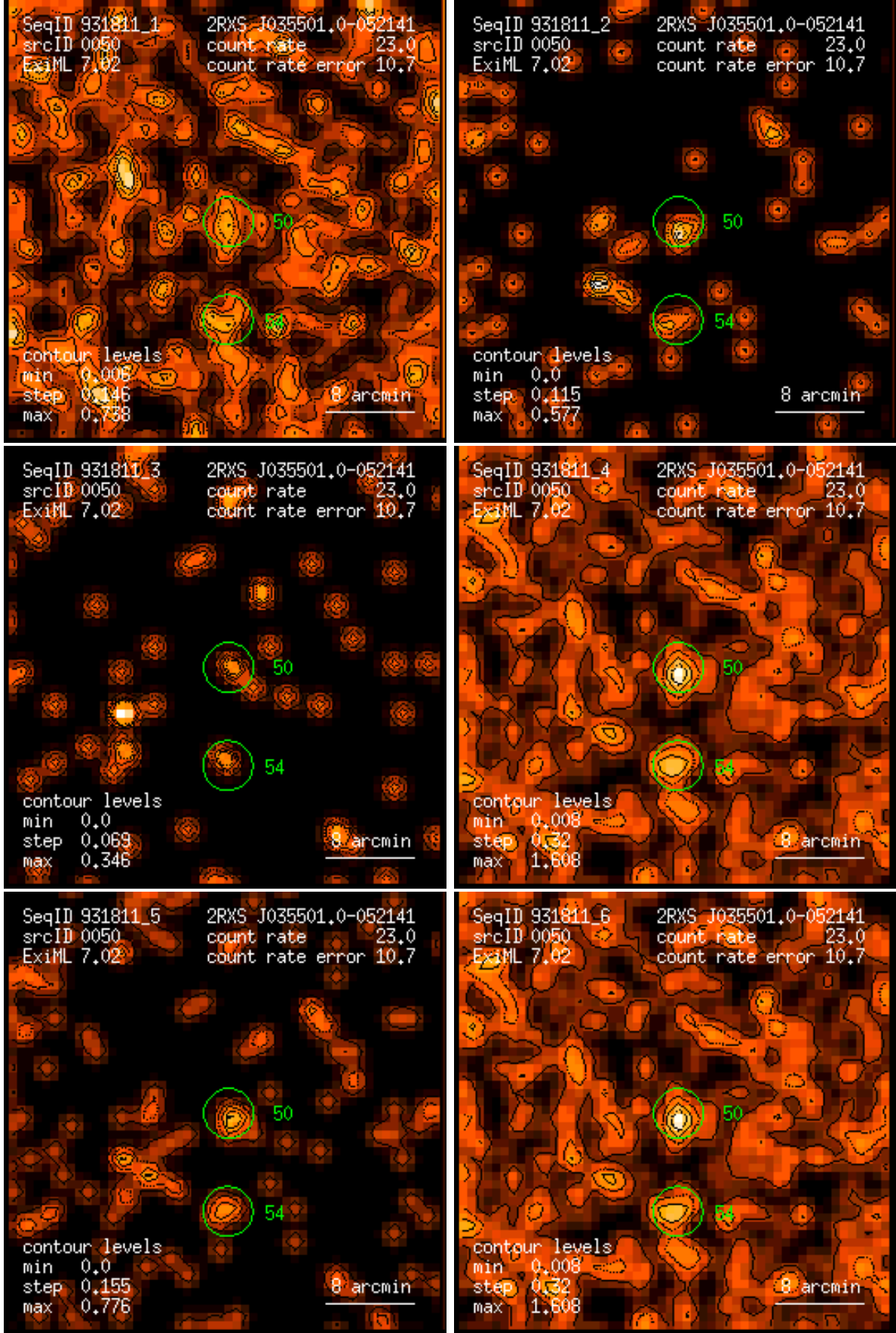
Figure 50: RASS 931811: detection 0050: band rate images, Gaussian filter: (1) PSPC channels 11 – 41, (2) 52 – 90, (3) 91 – 201, (4) 11 – 235, (5) 52 – 201, (6) 11 – 201. Broad band rates in counts/ks. Band rate contour levels in counts/ks/arcmin 2 .
