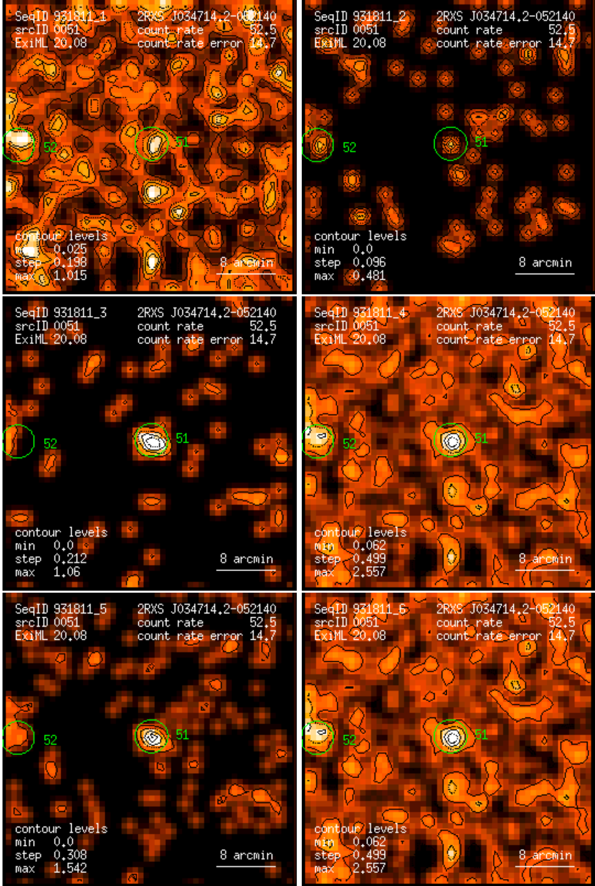
Figure 51: RASS 931811: detection 0051: band rate images, Gaussian filter: (1) PSPC channels 11 – 41, (2) 52 – 90, (3) 91 – 201, (4) 11 – 235, (5) 52 – 201, (6) 11 – 201. Broad band rates in counts/ks. Band rate contour levels in counts/ks/arcmin 2 .
