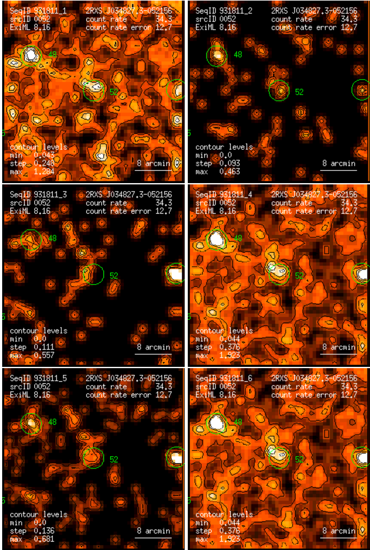
Figure 52: RASS 931811: detection 0052: band rate images, Gaussian filter: (1) PSPC channels 11 – 41, (2) 52 – 90, (3) 91 – 201, (4) 11 – 235, (5) 52 – 201, (6) 11 – 201. Broad band rates in counts/ks. Band rate contour levels in counts/ks/arcmin 2 .
