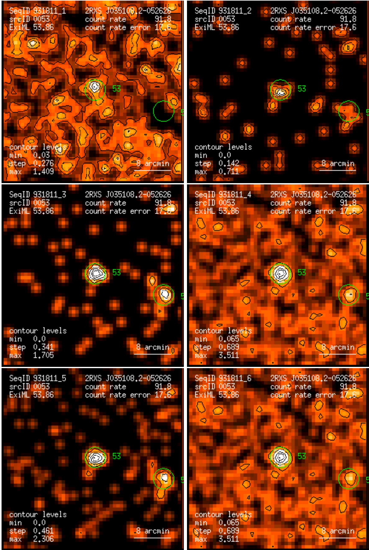
Figure 53: RASS 931811: detection 0053: band rate images, Gaussian filter: (1) PSPC channels 11 – 41, (2) 52 – 90, (3) 91 – 201, (4) 11 – 235, (5) 52 – 201, (6) 11 – 201. Broad band rates in counts/ks. Band rate contour levels in counts/ks/arcmin 2 .
