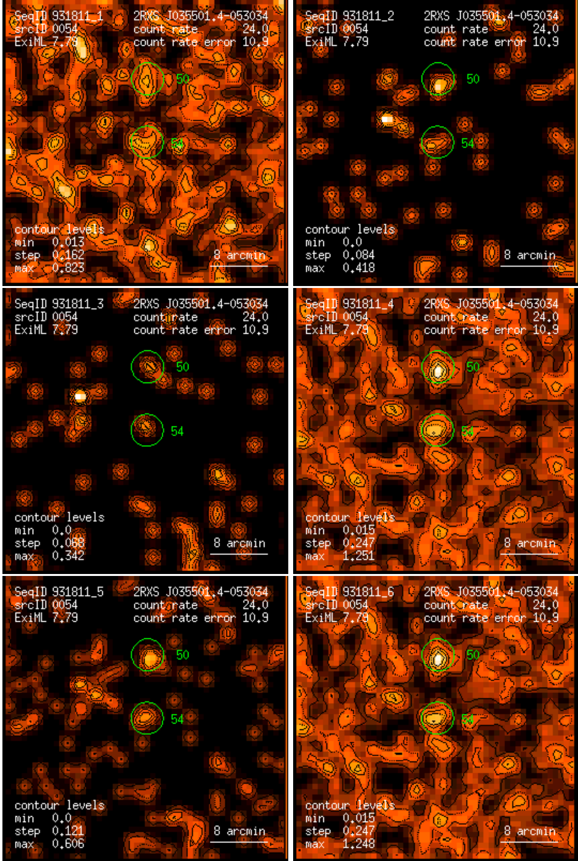
Figure 54: RASS 931811: detection 0054: band rate images, Gaussian filter: (1) PSPC channels 11 – 41, (2) 52 – 90, (3) 91 – 201, (4) 11 – 235, (5) 52 – 201, (6) 11 – 201. Broad band rates in counts/ks. Band rate contour levels in counts/ks/arcmin 2 .
