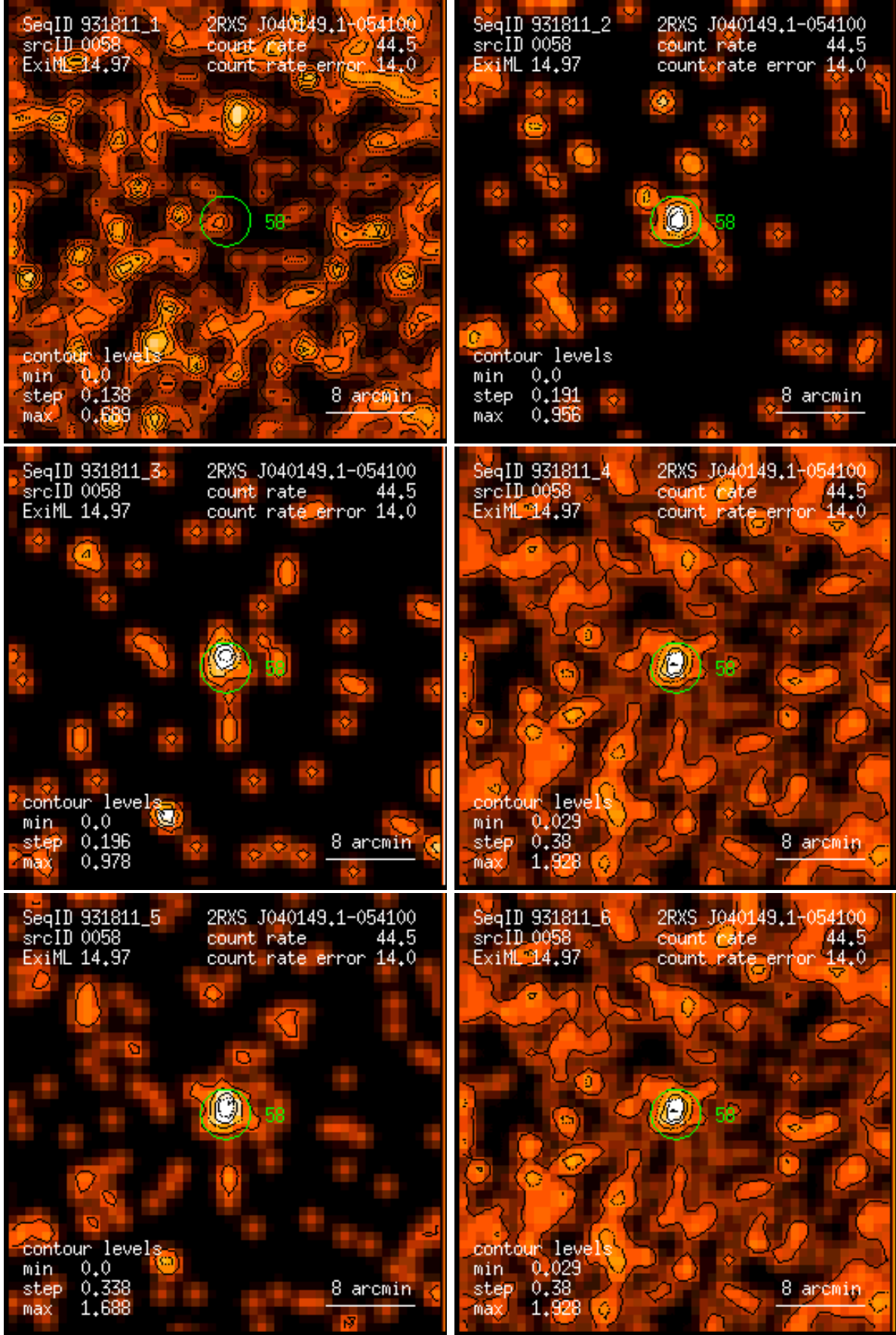
Figure 58: RASS 931811: detection 0058: band rate images, Gaussian filter: (1) PSPC channels 11 – 41, (2) 52 – 90, (3) 91 – 201, (4) 11 – 235, (5) 52 – 201, (6) 11 – 201. Broad band rates in counts/ks. Band rate contour levels in counts/ks/arcmin 2 .
