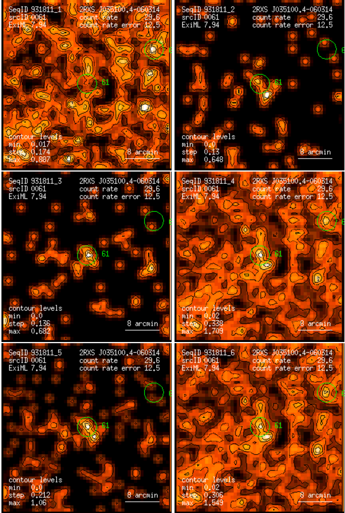
Figure 61: RASS 931811: detection 0061: band rate images, Gaussian filter: (1) PSPC channels 11 – 41, (2) 52 – 90, (3) 91 – 201, (4) 11 – 235, (5) 52 – 201, (6) 11 – 201. Broad band rates in counts/ks. Band rate contour levels in counts/ks/arcmin 2 .
