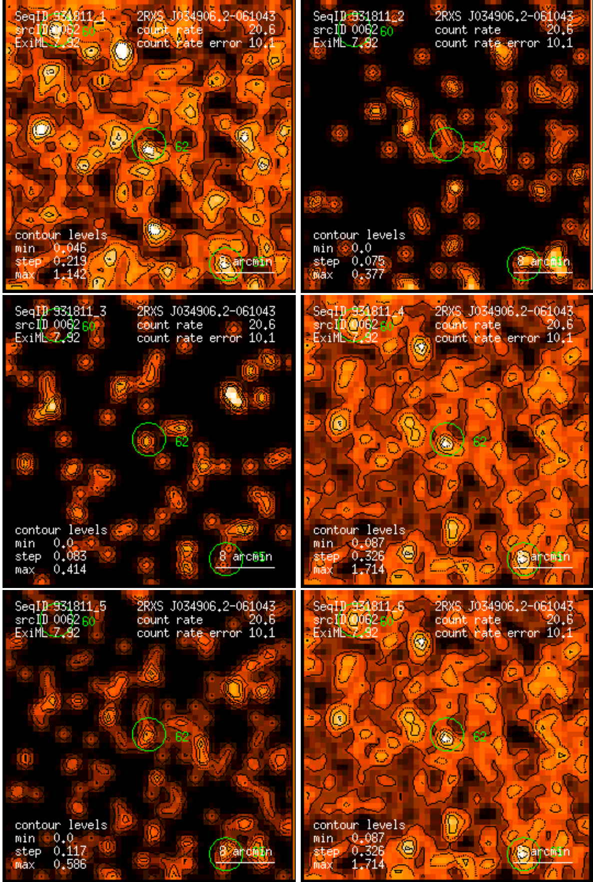
Figure 62: RASS 931811: detection 0062: band rate images, Gaussian filter: (1) PSPC channels 11 – 41, (2) 52 – 90, (3) 91 – 201, (4) 11 – 235, (5) 52 – 201, (6) 11 – 201. Broad band rates in counts/ks. Band rate contour levels in counts/ks/arcmin 2 .
