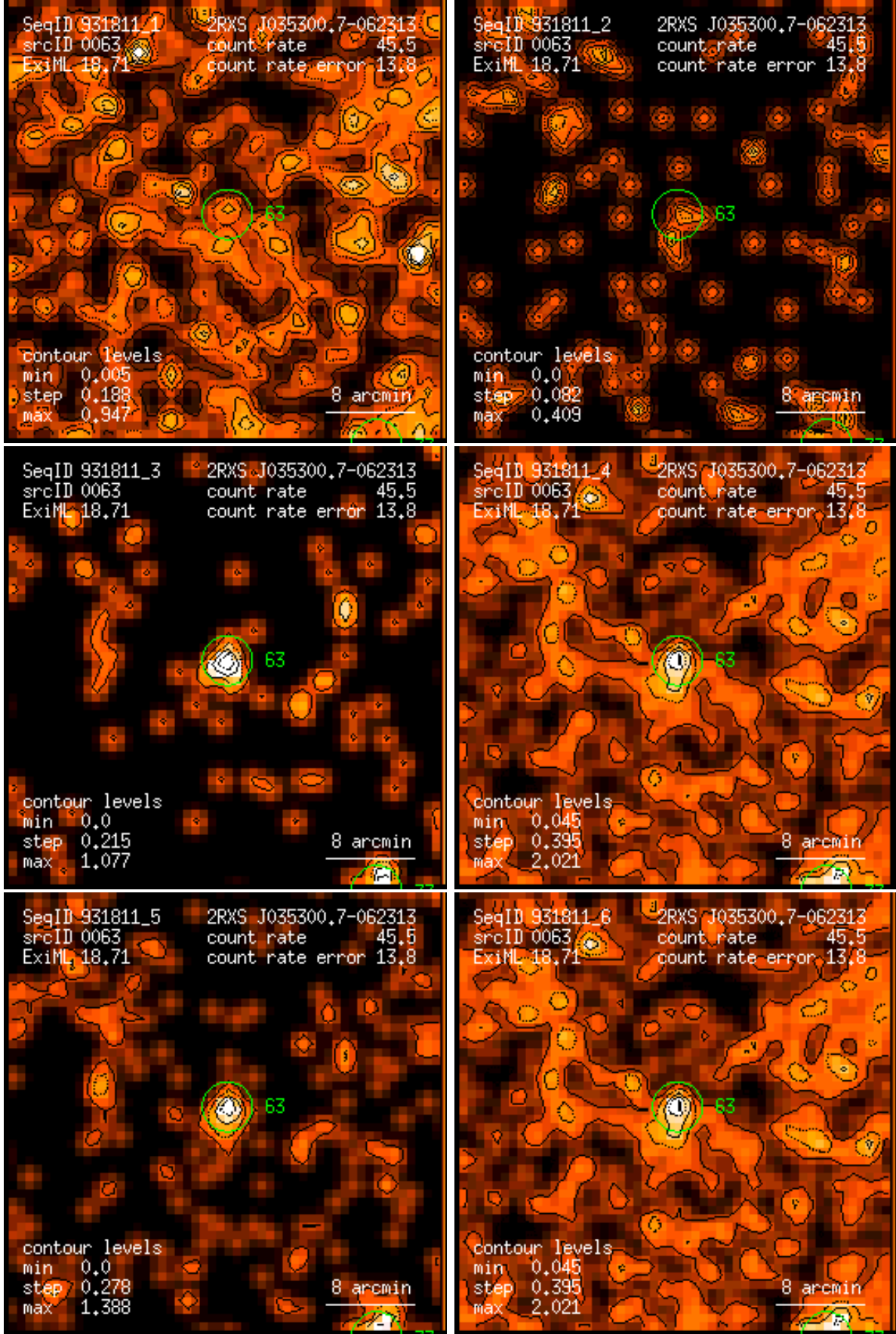
Figure 63: RASS 931811: detection 0063: band rate images, Gaussian filter: (1) PSPC channels 11 – 41, (2) 52 – 90, (3) 91 – 201, (4) 11 – 235, (5) 52 – 201, (6) 11 – 201. Broad band rates in counts/ks. Band rate contour levels in counts/ks/arcmin 2 .
