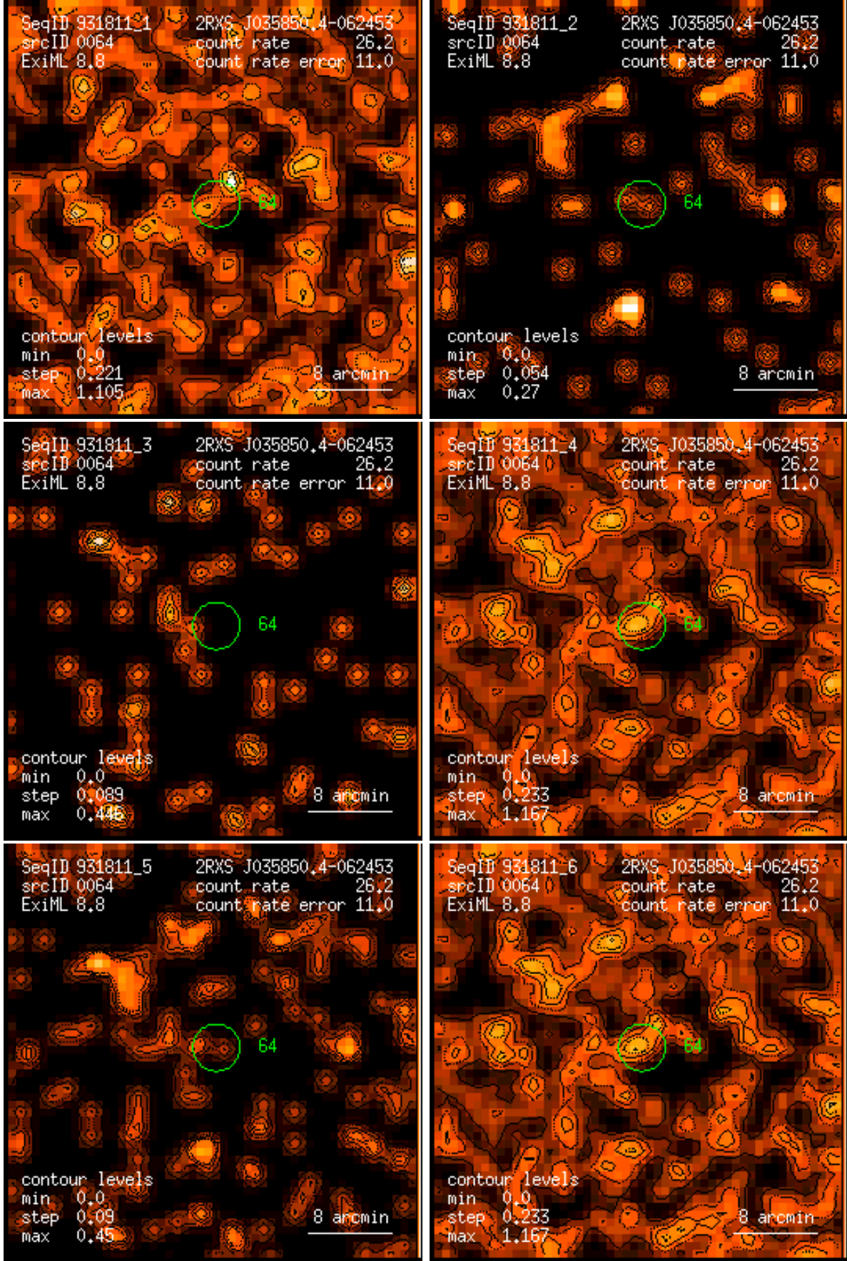
Figure 64: RASS 931811: detection 0064: band rate images, Gaussian filter: (1) PSPC channels 11 – 41, (2) 52 – 90, (3) 91 – 201, (4) 11 – 235, (5) 52 – 201, (6) 11 – 201. Broad band rates in counts/ks. Band rate contour levels in counts/ks/arcmin 2 .
