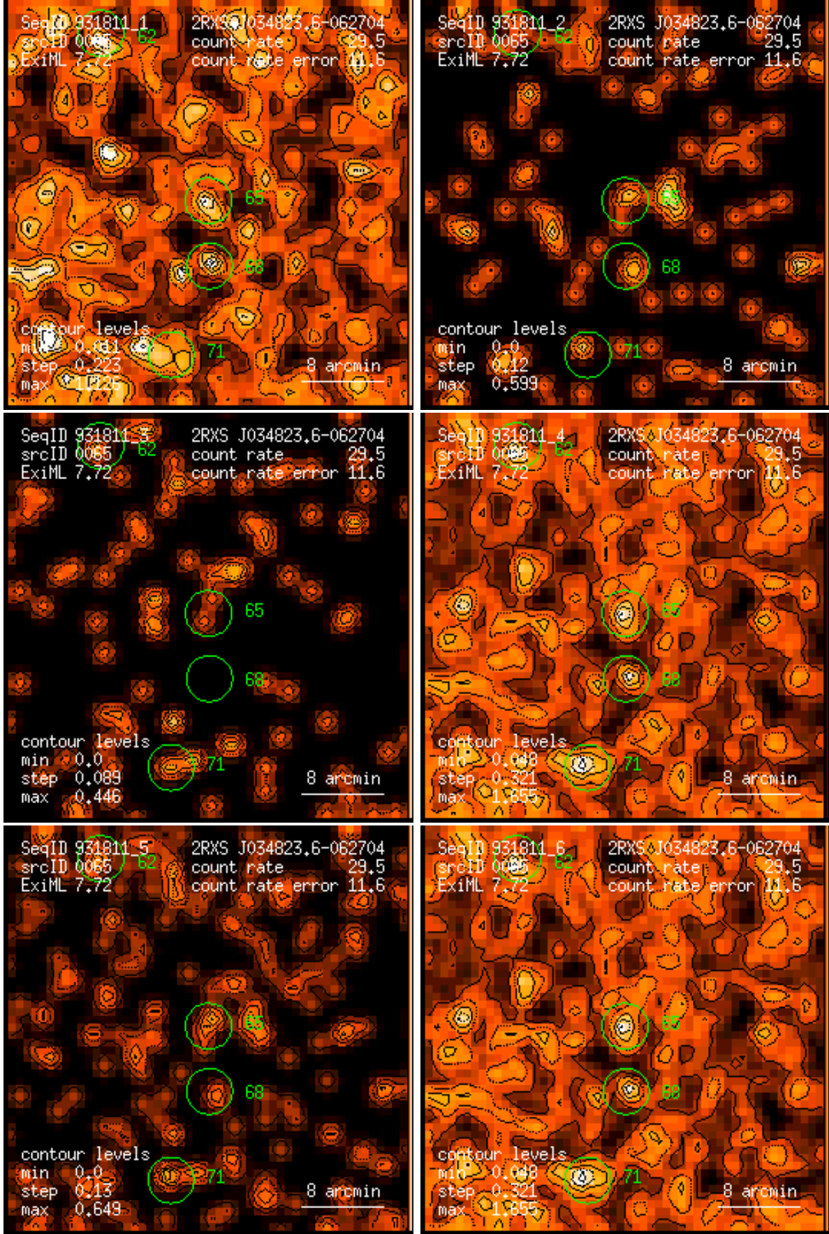
Figure 65: RASS 931811: detection 0065: band rate images, Gaussian filter: (1) PSPC channels 11 – 41, (2) 52 – 90, (3) 91 – 201, (4) 11 – 235, (5) 52 – 201, (6) 11 – 201. Broad band rates in counts/ks. Band rate contour levels in counts/ks/arcmin 2 .
