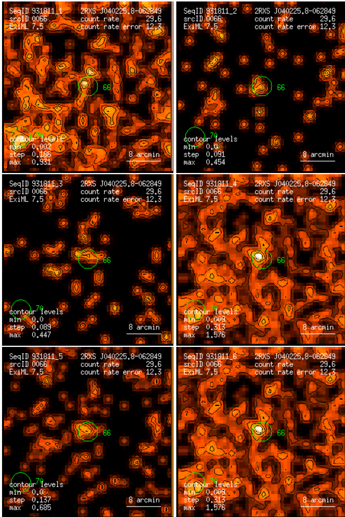
Figure 66: RASS 931811: detection 0066: band rate images, Gaussian filter: (1) PSPC channels 11 – 41, (2) 52 – 90, (3) 91 – 201, (4) 11 – 235, (5) 52 – 201, (6) 11 – 201. Broad band rates in counts/ks. Band rate contour levels in counts/ks/arcmin 2 .
