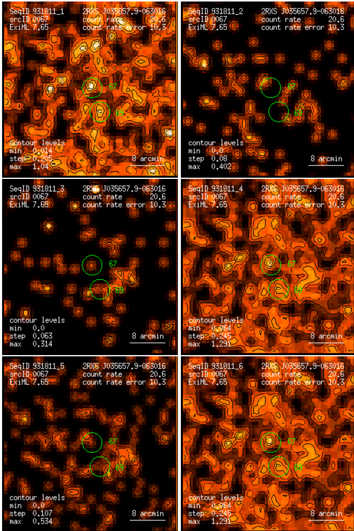
Figure 67: RASS 931811: detection 0067: band rate images, Gaussian filter: (1) PSPC channels 11 – 41, (2) 52 – 90, (3) 91 – 201, (4) 11 – 235, (5) 52 – 201, (6) 11 – 201. Broad band rates in counts/ks. Band rate contour levels in counts/ks/arcmin 2 .
