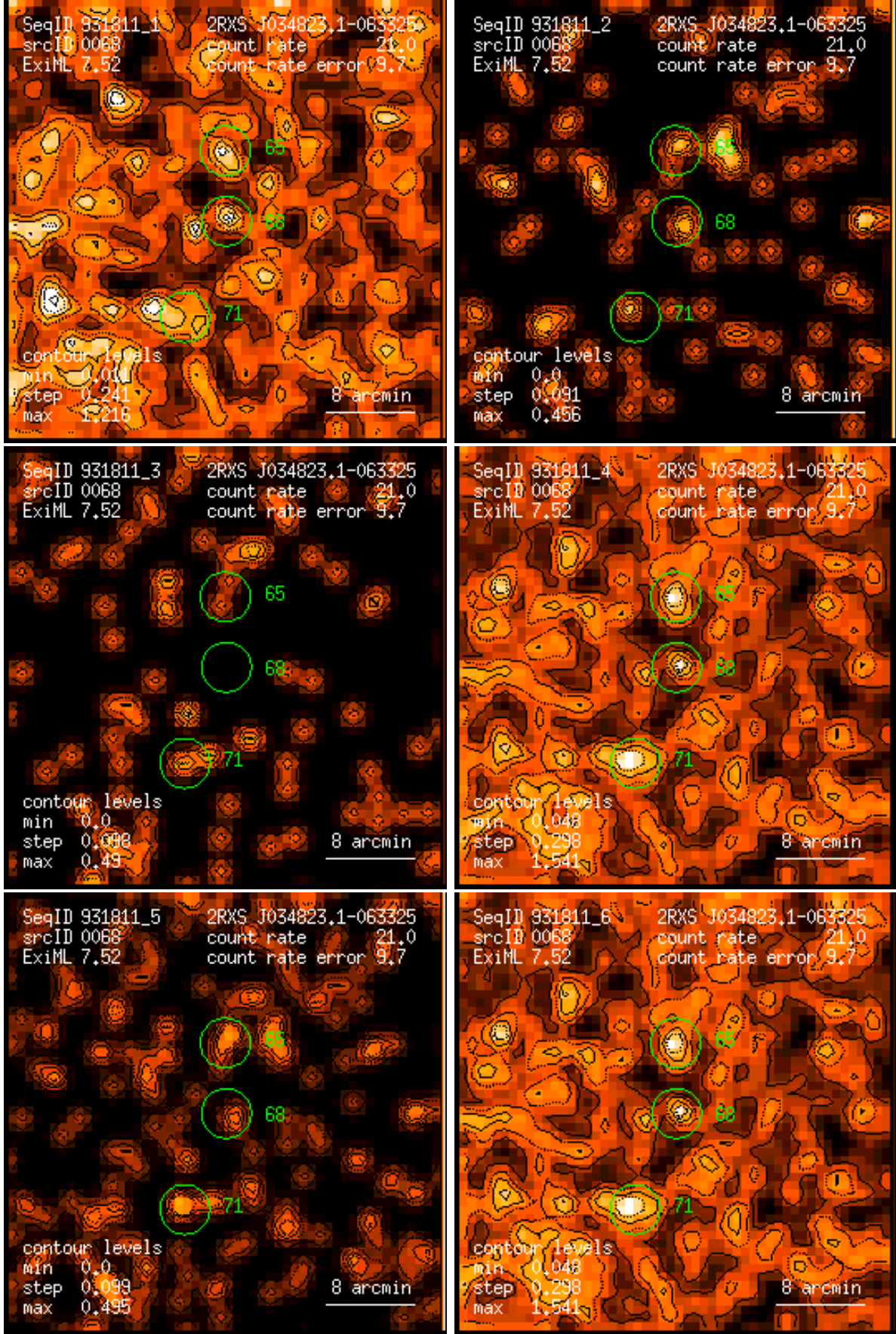
Figure 68: RASS 931811: detection 0068: band rate images, Gaussian filter: (1) PSPC channels 11 – 41, (2) 52 – 90, (3) 91 – 201, (4) 11 – 235, (5) 52 – 201, (6) 11 – 201. Broad band rates in counts/ks. Band rate contour levels in counts/ks/arcmin 2 .
