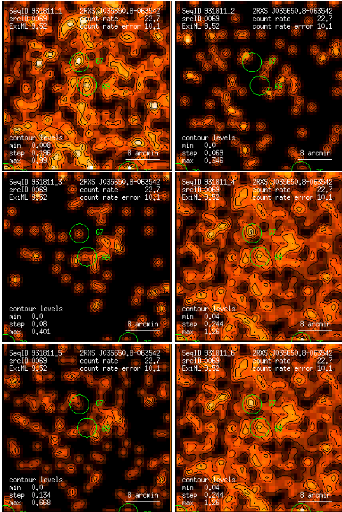
Figure 69: RASS 931811: detection 0069: band rate images, Gaussian filter: (1) PSPC channels 11 – 41, (2) 52 – 90, (3) 91 – 201, (4) 11 – 235, (5) 52 – 201, (6) 11 – 201. Broad band rates in counts/ks. Band rate contour levels in counts/ks/arcmin 2 .
