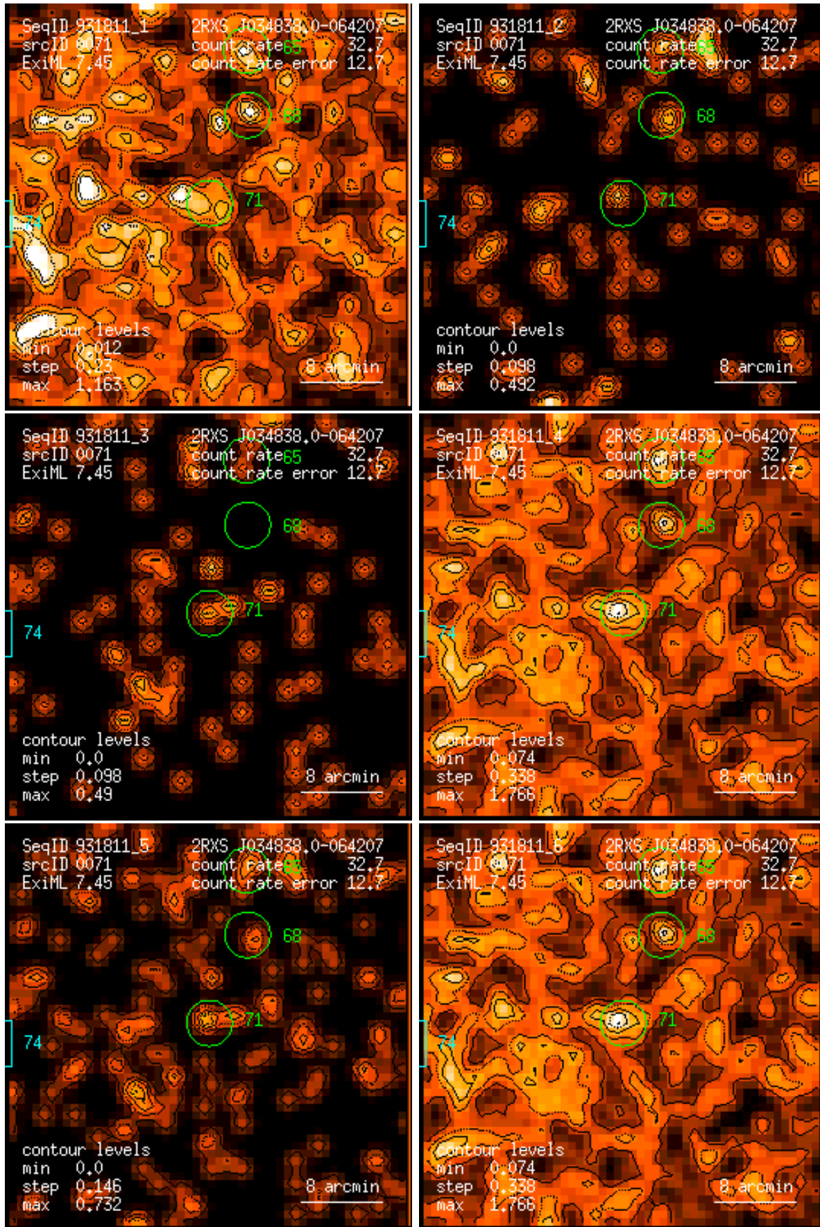
Figure 71: RASS 931811: detection 0071: band rate images, Gaussian filter: (1) PSPC channels 11 – 41, (2) 52 – 90, (3) 91 – 201, (4) 11 – 235, (5) 52 – 201, (6) 11 – 201. Broad band rates in counts/ks. Band rate contour levels in counts/ks/arcmin 2 .
