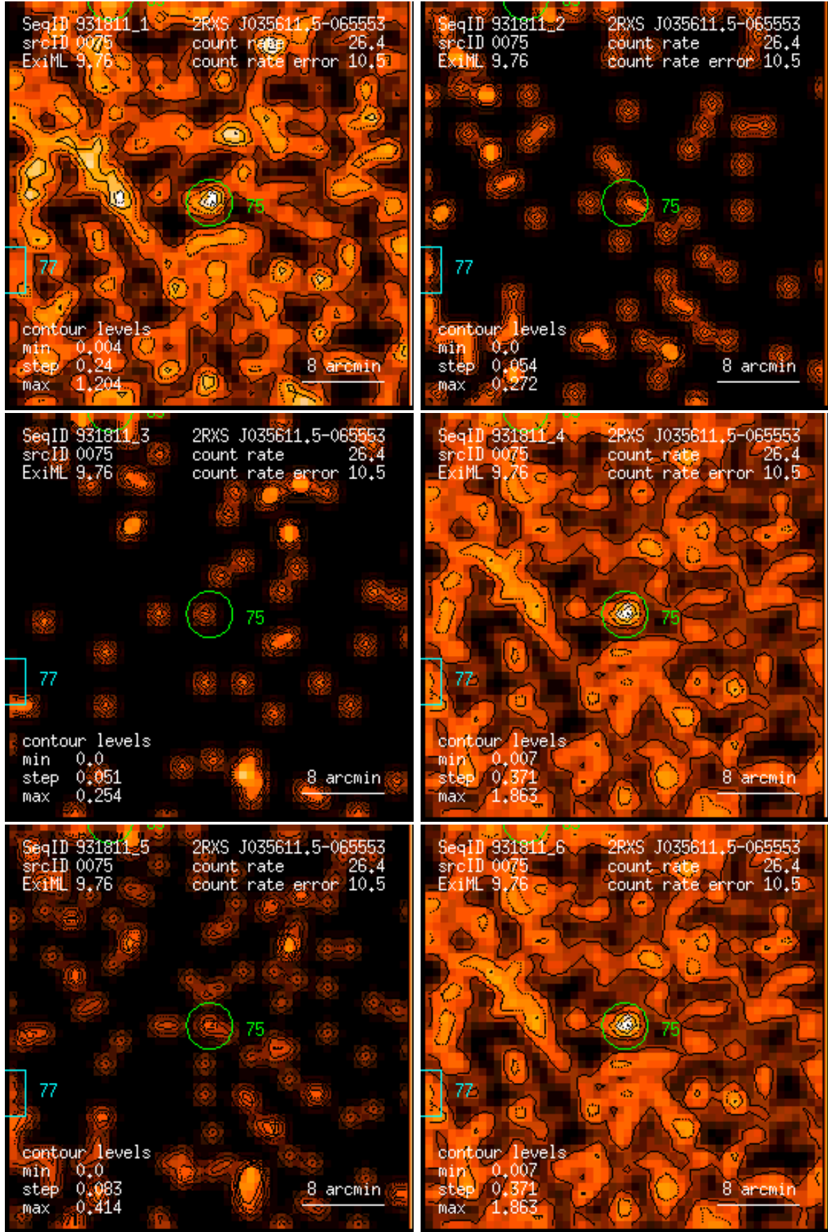
Figure 75: RASS 931811: detection 0075: band rate images, Gaussian filter: (1) PSPC channels 11 – 41, (2) 52 – 90, (3) 91 – 201, (4) 11 – 235, (5) 52 – 201, (6) 11 – 201. Broad band rates in counts/ks. Band rate contour levels in counts/ks/arcmin 2 .
