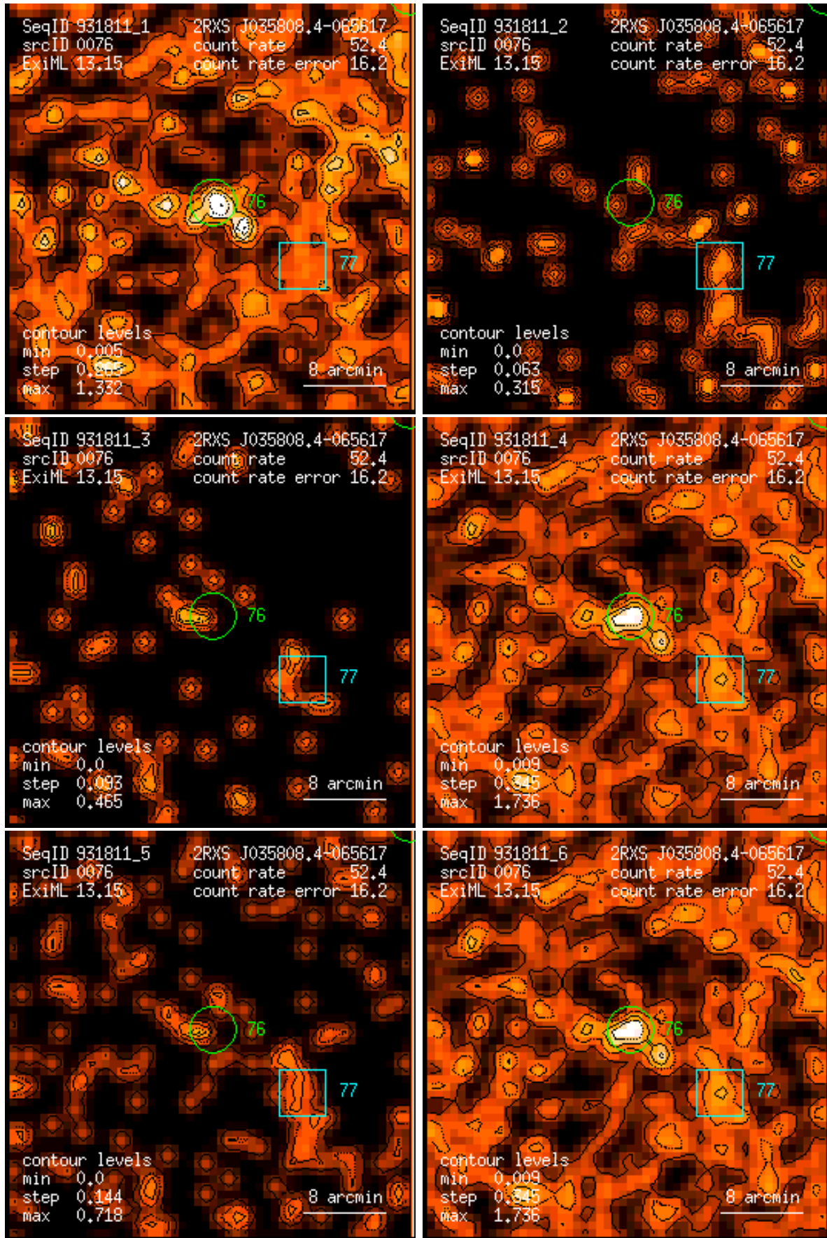
Figure 76: RASS 931811: detection 0076: band rate images, Gaussian filter: (1) PSPC channels 11 – 41, (2) 52 – 90, (3) 91 – 201, (4) 11 – 235, (5) 52 – 201, (6) 11 – 201. Broad band rates in counts/ks. Band rate contour levels in counts/ks/arcmin 2 .
