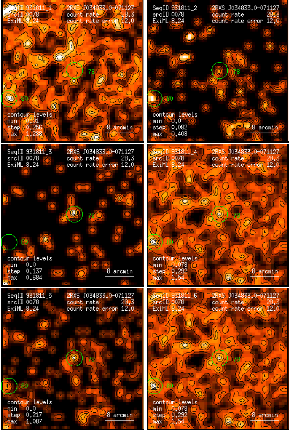
Figure 78: RASS 931811: detection 0078: band rate images, Gaussian filter: (1) PSPC channels 11 – 41, (2) 52 – 90, (3) 91 – 201, (4) 11 – 235, (5) 52 – 201, (6) 11 – 201. Broad band rates in counts/ks. Band rate contour levels in counts/ks/arcmin 2 .
