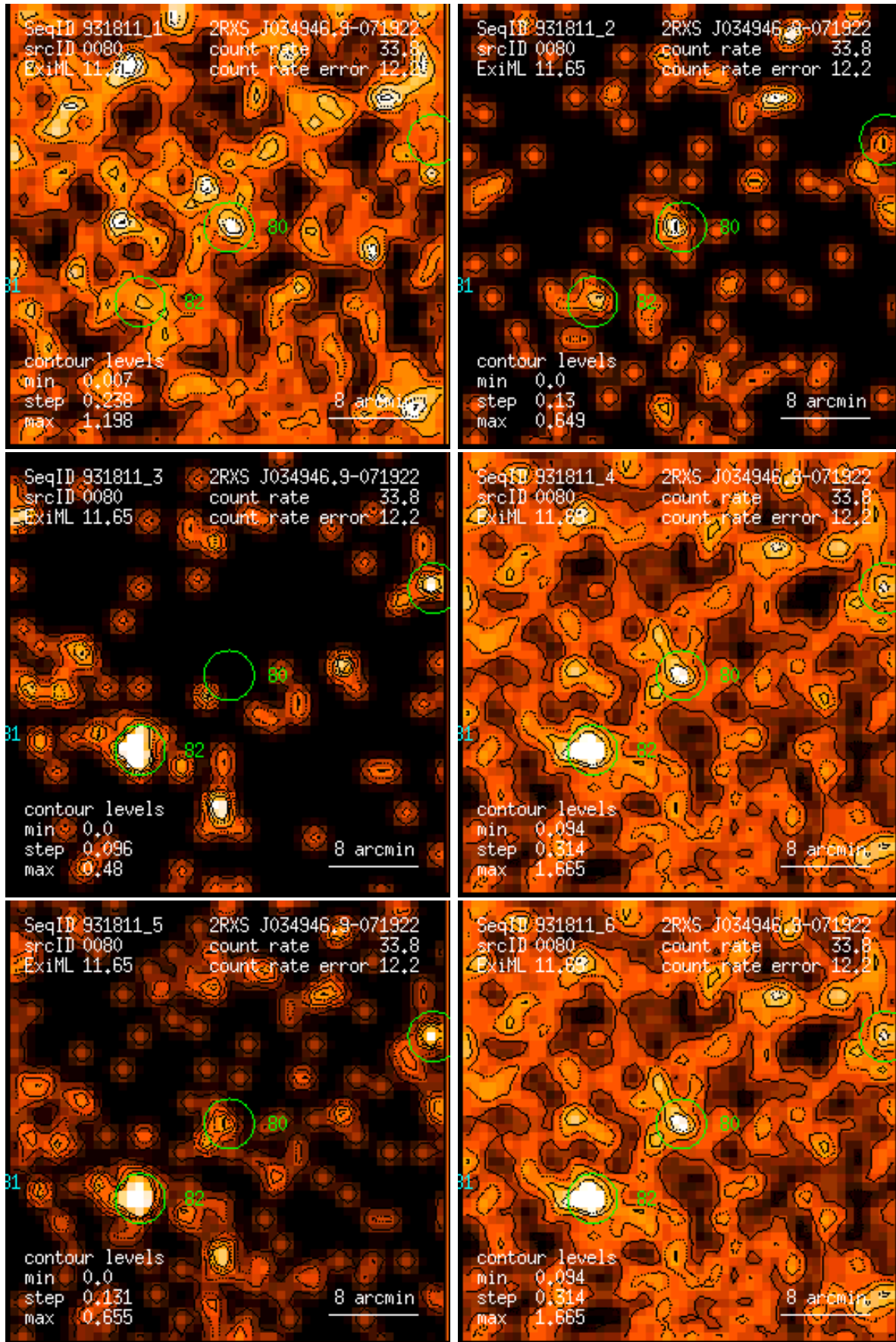
Figure 80: RASS 931811: detection 0080: band rate images, Gaussian filter: (1) PSPC channels 11 – 41, (2) 52 – 90, (3) 91 – 201, (4) 11 – 235, (5) 52 – 201, (6) 11 – 201. Broad band rates in counts/ks. Band rate contour levels in counts/ks/arcmin 2 .
