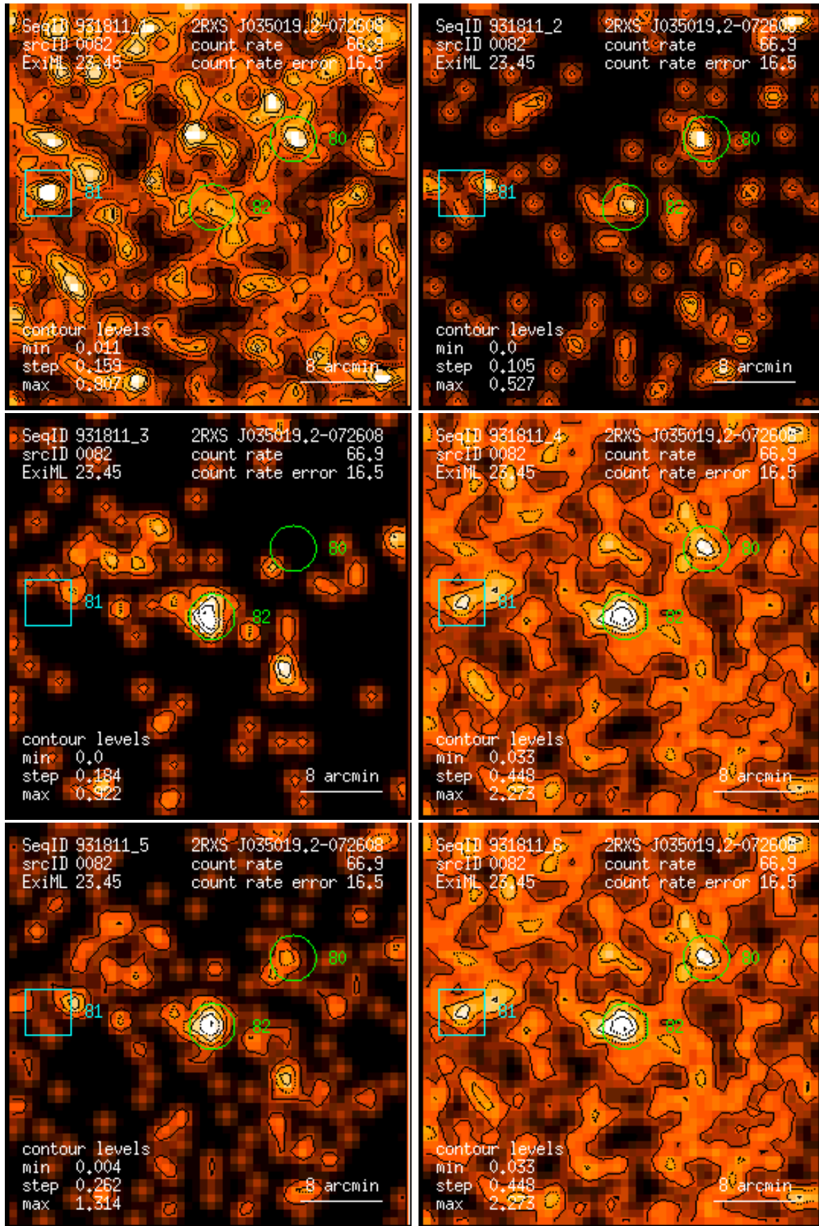
Figure 82: RASS 931811: detection 0082: band rate images, Gaussian filter: (1) PSPC channels 11 – 41, (2) 52 – 90, (3) 91 – 201, (4) 11 – 235, (5) 52 – 201, (6) 11 – 201. Broad band rates in counts/ks. Band rate contour levels in counts/ks/arcmin 2 .
