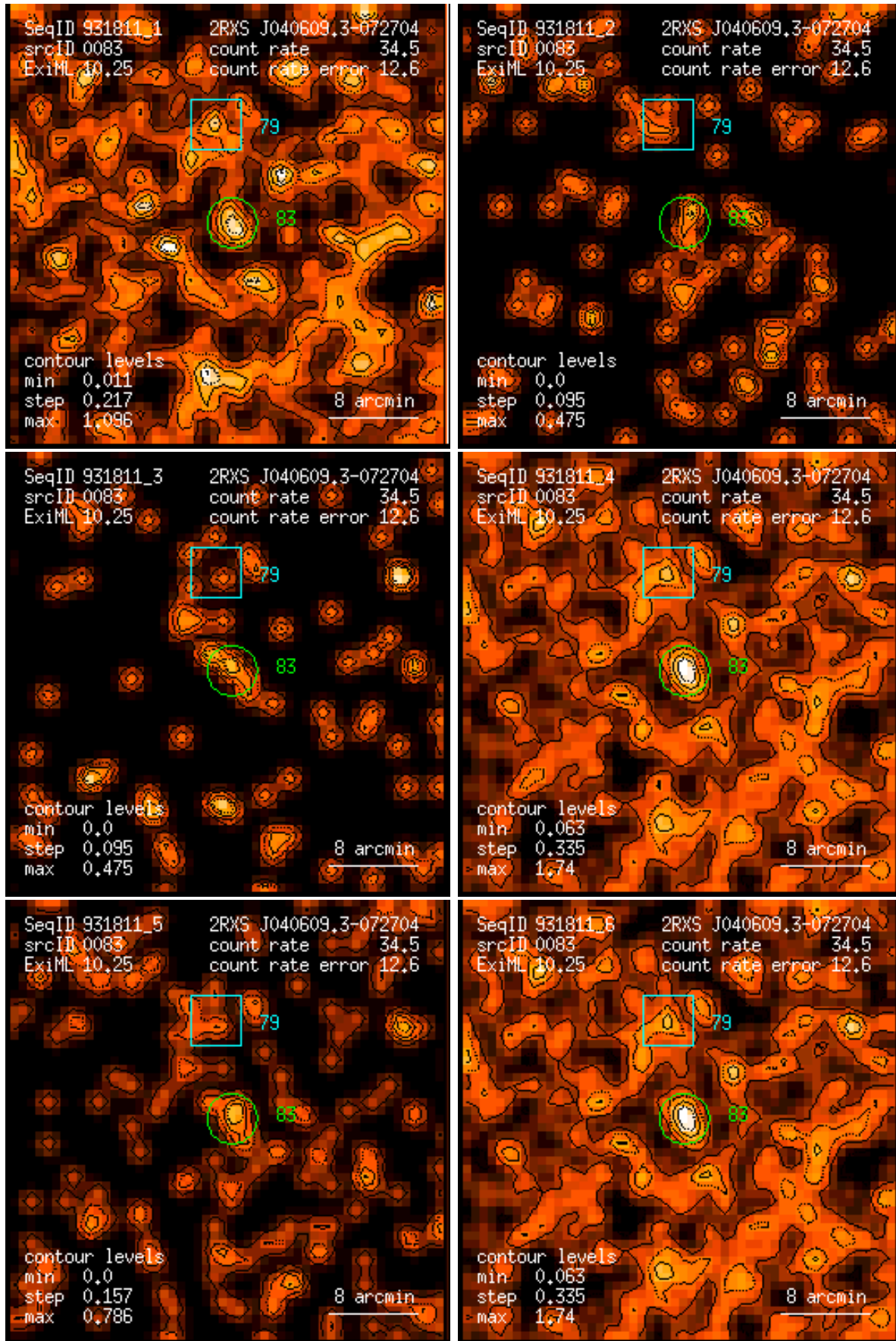
Figure 83: RASS 931811: detection 0083: band rate images, Gaussian filter: (1) PSPC channels 11 – 41, (2) 52 – 90, (3) 91 – 201, (4) 11 – 235, (5) 52 – 201, (6) 11 – 201. Broad band rates in counts/ks. Band rate contour levels in counts/ks/arcmin 2 .
