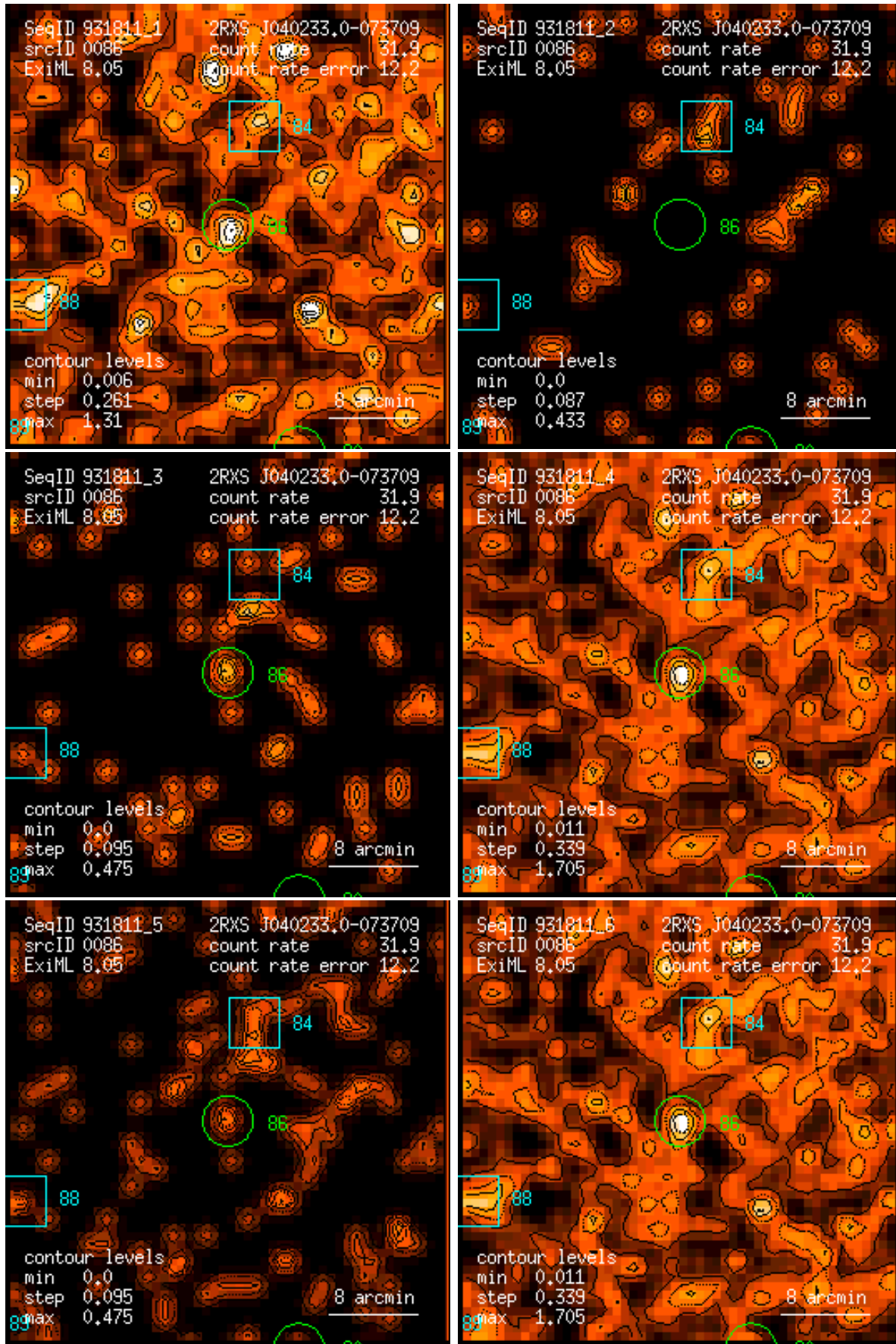
Figure 86: RASS 931811: detection 0086: band rate images, Gaussian filter: (1) PSPC channels 11 – 41, (2) 52 – 90, (3) 91 – 201, (4) 11 – 235, (5) 52 – 201, (6) 11 – 201. Broad band rates in counts/ks. Band rate contour levels in counts/ks/arcmin 2 .
