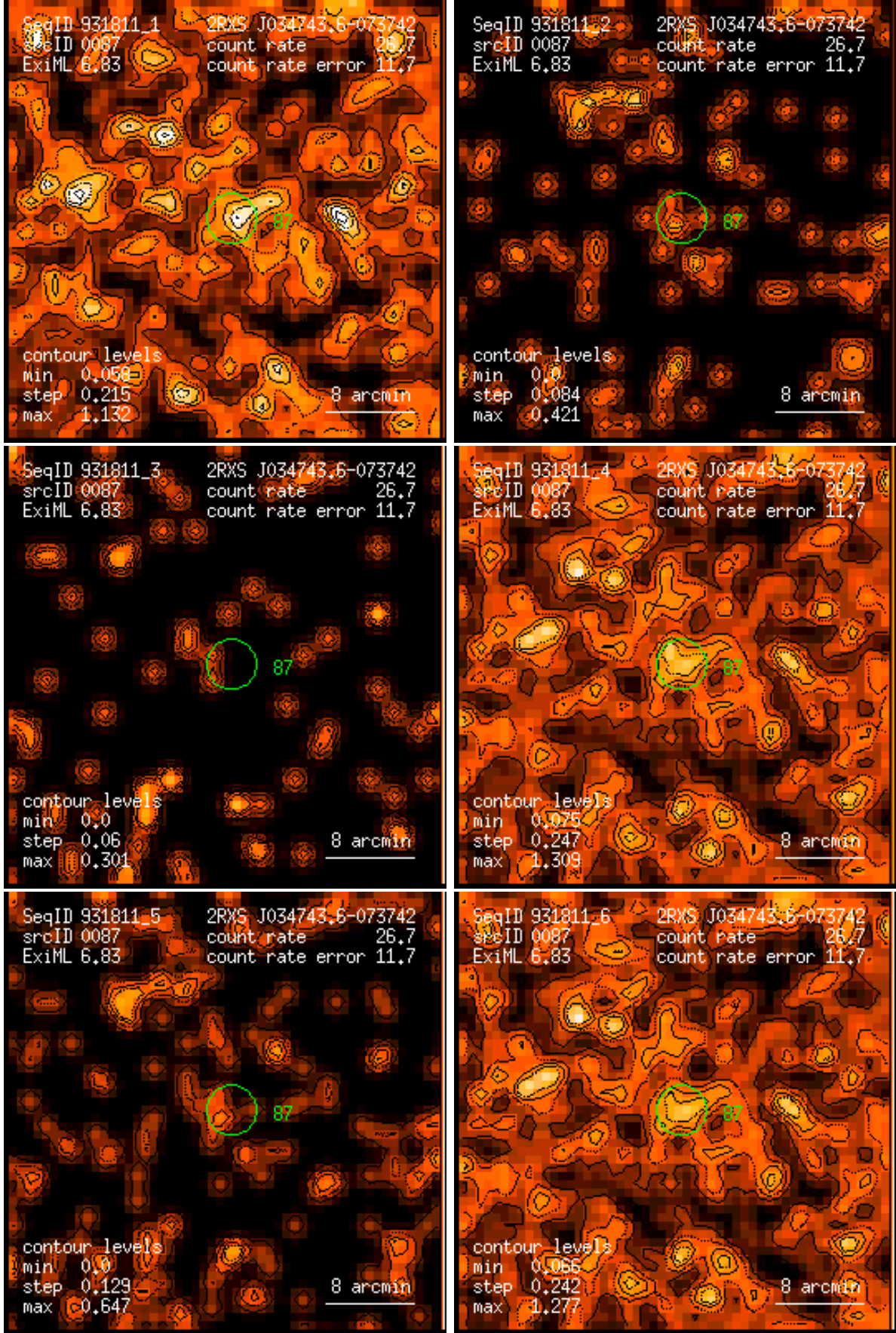
Figure 87: RASS 931811: detection 0087: band rate images, Gaussian filter: (1) PSPC channels 11 – 41, (2) 52 – 90, (3) 91 – 201, (4) 11 – 235, (5) 52 – 201, (6) 11 – 201. Broad band rates in counts/ks. Band rate contour levels in counts/ks/arcmin 2 .
