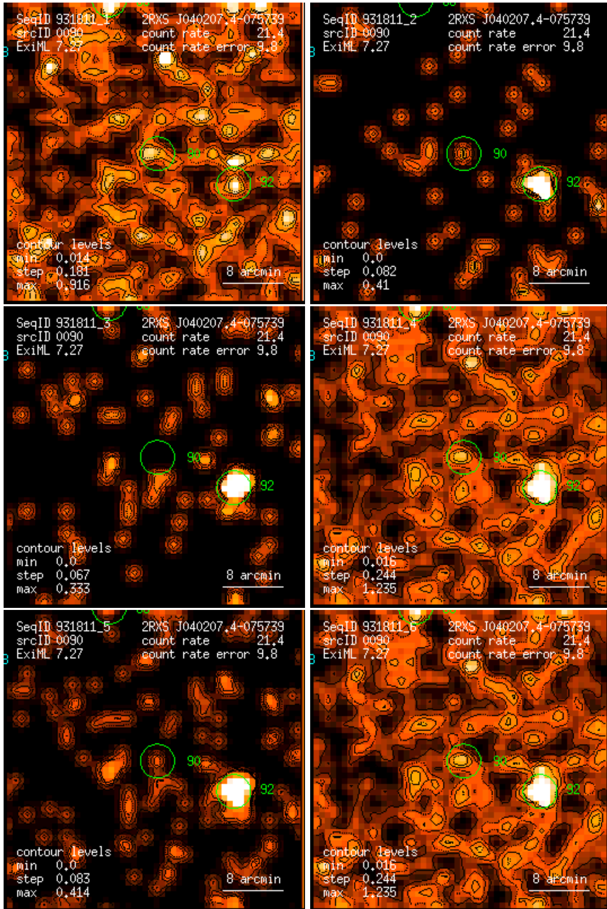
Figure 90: RASS 931811: detection 0090: band rate images, Gaussian filter: (1) PSPC channels 11 – 41, (2) 52 – 90, (3) 91 – 201, (4) 11 – 235, (5) 52 – 201, (6) 11 – 201. Broad band rates in counts/ks. Band rate contour levels in counts/ks/arcmin 2 .
