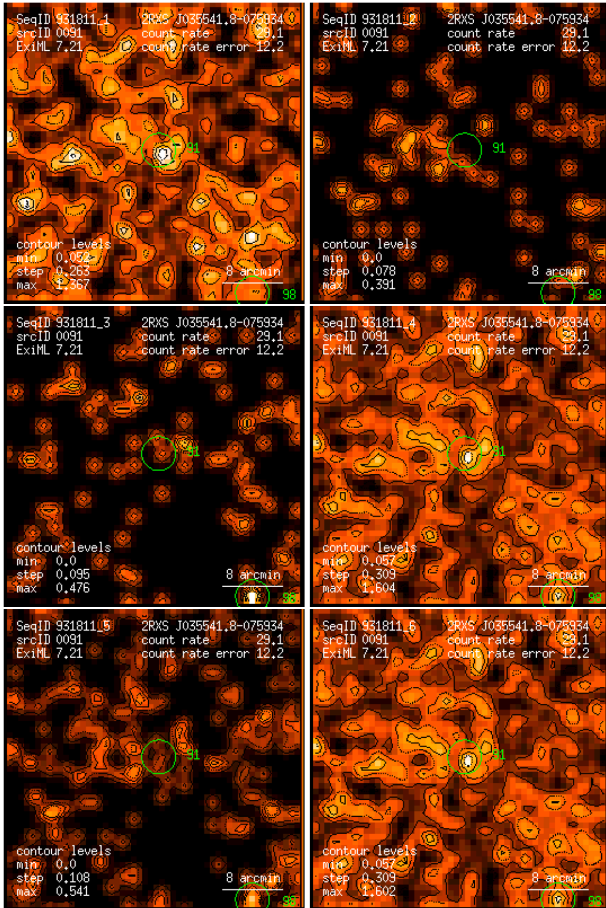
Figure 91: RASS 931811: detection 0091: band rate images, Gaussian filter: (1) PSPC channels 11 – 41, (2) 52 – 90, (3) 91 – 201, (4) 11 – 235, (5) 52 – 201, (6) 11 – 201. Broad band rates in counts/ks. Band rate contour levels in counts/ks/arcmin 2 .
