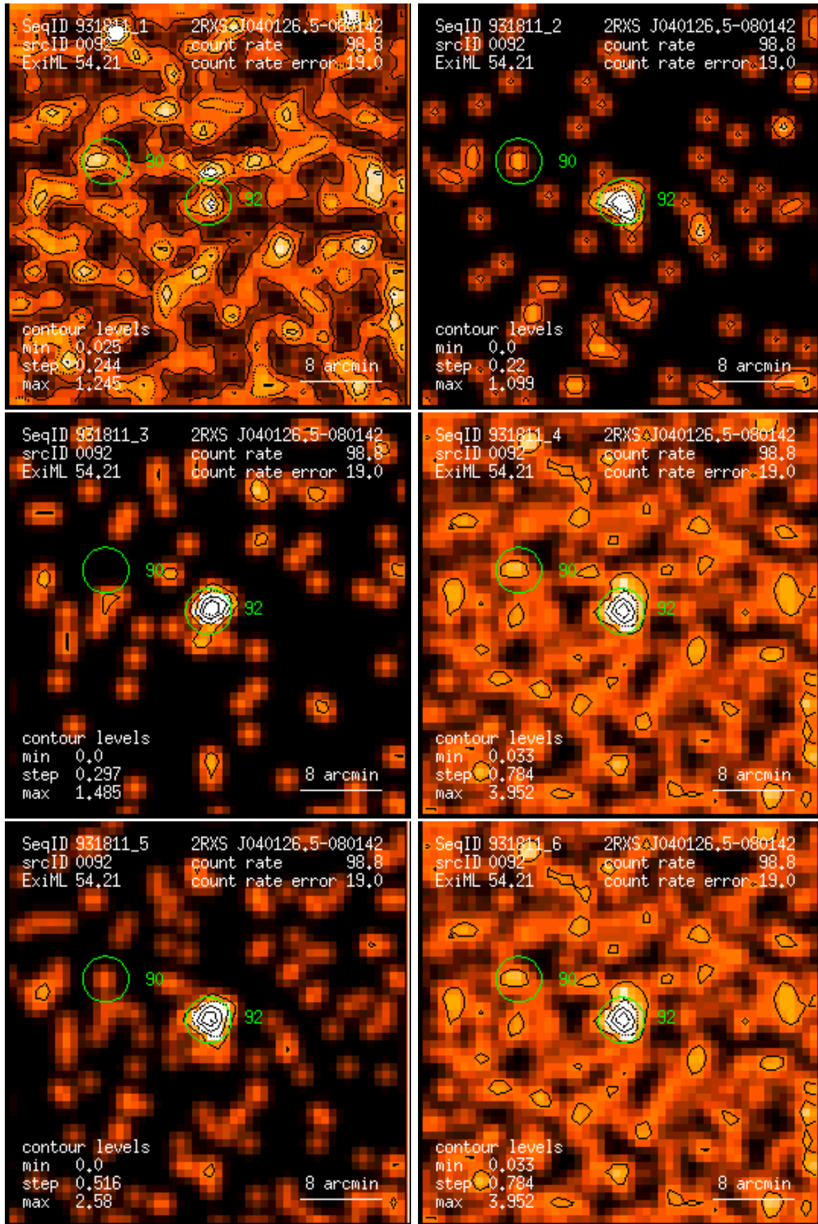
Figure 92: RASS 931811: detection 0092: band rate images, Gaussian filter: (1) PSPC channels 11 – 41, (2) 52 – 90, (3) 91 – 201, (4) 11 – 235, (5) 52 – 201, (6) 11 – 201. Broad band rates in counts/ks. Band rate contour levels in counts/ks/arcmin 2 .
