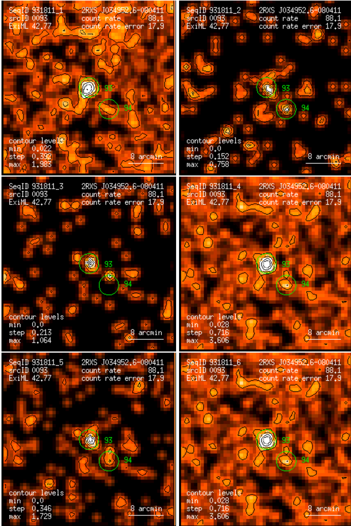
Figure 93: RASS 931811: detection 0093: band rate images, Gaussian filter: (1) PSPC channels 11 – 41, (2) 52 – 90, (3) 91 – 201, (4) 11 – 235, (5) 52 – 201, (6) 11 – 201. Broad band rates in counts/ks. Band rate contour levels in counts/ks/arcmin 2 .
