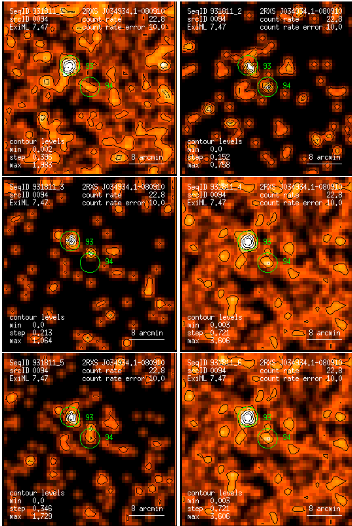
Figure 94: RASS 931811: detection 0094: band rate images, Gaussian filter: (1) PSPC channels 11 – 41, (2) 52 – 90, (3) 91 – 201, (4) 11 – 235, (5) 52 – 201, (6) 11 – 201. Broad band rates in counts/ks. Band rate contour levels in counts/ks/arcmin 2 .
