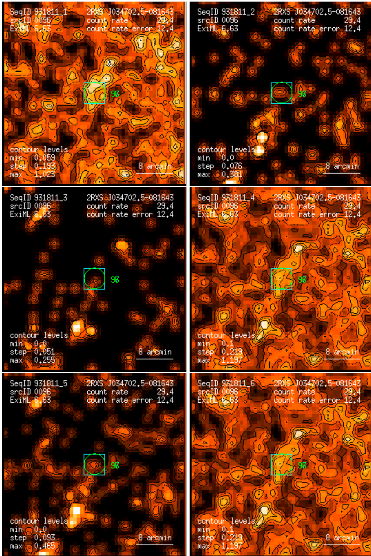
Figure 96: RASS 931811: detection 0096: band rate images, Gaussian filter: (1) PSPC channels 11 – 41, (2) 52 – 90, (3) 91 – 201, (4) 11 – 235, (5) 52 – 201, (6) 11 – 201. Broad band rates in counts/ks. Band rate contour levels in counts/ks/arcmin 2 .
